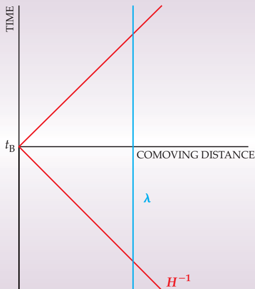
Figure 3. Pre-Big Bang cosmology. Before the bounce time t_B , the universe is contracting. The bounce itself is a singular transition between the contracting phase and the usual radiation phase of standard Big Bang cosmology. As in inflationary cosmology, the scale of a fluctuation (blue) starts out sub-Hubble, crosses the Hubble length (red), and evolves for a long time on super-Hubble scales before recrossing the Hubble length. The behavior of the Hubble length and a fixed wavelength appear particularly simple in terms of “comoving” distance, for which the expansion or contraction of space is factored out.
