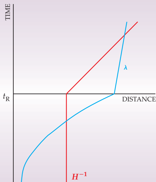
Figure 2. Fluctuation evolution in inflationary cosmology. The period of accelerated expansion ends at the so-called reheating time t_R , when the inflation field decays and regular matter is generated. After reheating comes the radiation-dominated phase of standard cosmology. The red line indicates the Hubble length, which is constant during the exponential expansion but increases linearly after t_R . The blue line denotes the evolution of a structure with wavelength \lambda . Initially, the wavelength is less than the Hubble length. Eventually, it exceeds the Hubble length and then evolves for a long time on super-Hubble scales. At late times the Hubble length catches up to the fluctuation wavelength. After that final crossing, the fluctuations oscillate. The evolution of fluctuations from sub-Hubble to super-Hubble and back is a common feature of alternatives to inflation that replicate inflation's success in generating fluctuations on cosmological scales.
