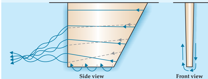
Figure 2. Vortex formation by the keel. Unless the boat is sailing straight ahead, there's a pressure difference between the two sides of the keel. As a result, the water flow angles down on the high-pressure (lower water-speed) side and up on the low-pressure side, creating a twist in the flow that generates vortices behind the bottom rear of the keel.
