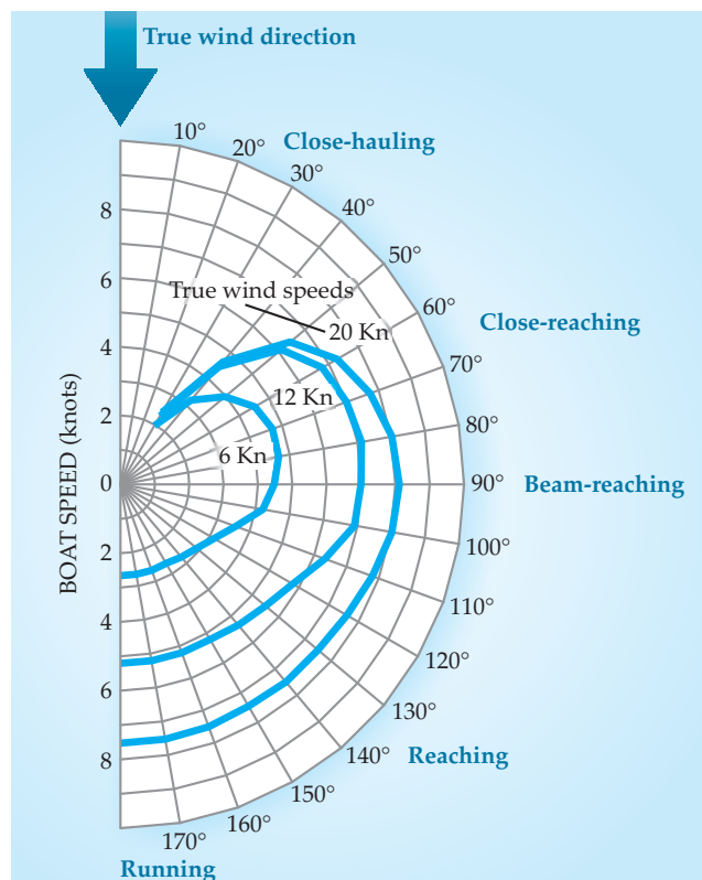
Figure 5. Speeds predicted by a computer model 5 for a 10-meter-long cruising sailboat, plotted for three different wind speeds from 6 to 20 knots as a function of the angle of the boat's motion relative to the wind direction. (10 knots = 18.5 km/h.) An angle of 180° means the boat is "running" with the wind directly at its back. The fastest speeds are predicted when the boat is "beam reaching," that is, moving at about 90° to the wind. The boat even makes some progress when it's "close hauling" almost directly into the wind.
