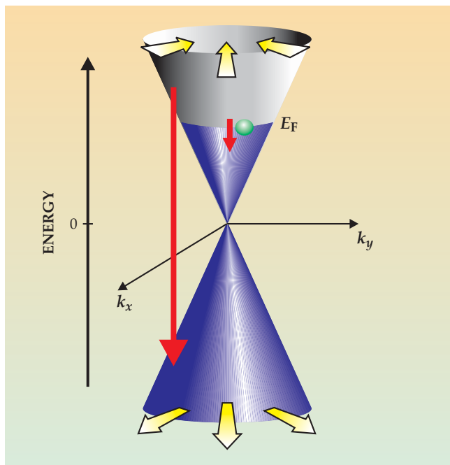
Figure 2. The electron-correlation physics of graphene, with its linear dispersion relation, differs from that of an ordinary two-dimensional semiconductor in two ways: First, electron states in conduction and valence bands have opposite chirality (see box 2), as indicated by yellow arrows. Interaction energies are lowered when most electrons have the same chirality, just as interaction energies in ferromagnets are lowered when most particles have the same spin. Second, an electron (green dot) at graphene's Fermi energy E_F carries with it a fluctuating polarization cloud that gives rise to both intragap (short red arrow) and interband (long red arrow) transitions. In ordinary 2D electron or hole systems, the contribution to polarization from interband transitions can be captured by using the appropriate dielectric constant and does not need to be considered explicitly. (Adapted from M. Polini et al., Solid State Commun. 143 , 58, 2007.)
