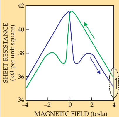
Figure 2. Magnetic dependence of the electrical resistance seen at an interface between lanthanum aluminate and strontium titanate. Arrows indicate data taken as the magnetic field is being raised or lowered. Measurements continued to higher fields are not shown, as suggested by the dashed circle. The butterfly-shaped hysteresis loop suggests the presence of ferromagnetism. (Adapted from ref. 2.)
