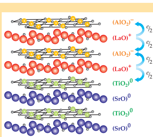
Figure 1. Layered structure of the interface between lanthanum aluminate and strontium titanate, showing the alternating planes of atoms. La, Al, Sr, Ti, and O atoms are shown as orange, yellow, purple, green, and gray, respectively. Arrows labeled e/2 indicate the charge transfer between LaO and AlO 2 layers because of ionic bonding. When the LaO layer is grown atop the originally neutral TiO 2 layer, there is a net charge transfer of e/2 per unit cell to that layer. (Adapted from refs. 3 and 10.)
