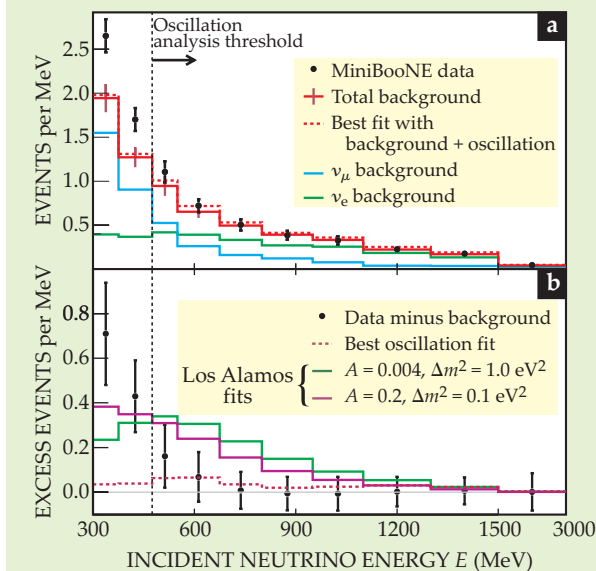
Figure 3. (a) MiniBooNE's observed distribution of quasi-elastic \nu_e collisions as a function of the neutrino's energy, plotted with expected backgrounds from masquerading \nu_\mu collisions and from real \nu_e contamination in the neutrino beam. Data for energy E above the indicated analysis threshold were used to determine the parameters of a model that allows neutrino oscillation on top of background. (b) The background-subtracted distribution, compared with predictions from two alternative neutrino-oscillation fits to the old Los Alamos results under scrutiny. They fit neither the data above the analysis threshold nor the unexpected excess below it. The best MiniBooNE oscillation parameters, incompatible with the Los Alamos results, do fit the data above the analysis threshold. But those data are adequately described by background alone. And none of the neutrino-oscillation fits explain the surprising low-energy excess. (Adapted from ref. 1.)
