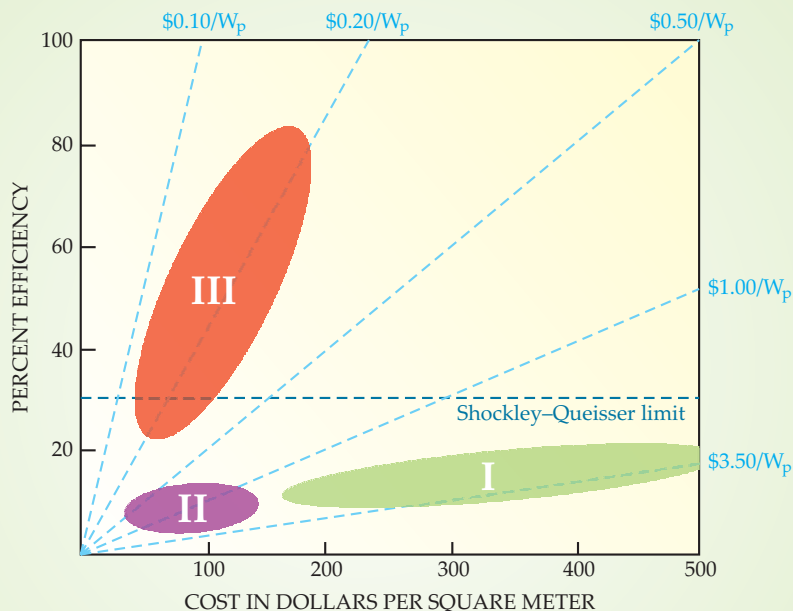
Figure 3. The three generations of solar cells. First-generation cells are based on expensive silicon wafers and make up 85% of the current commercial market. Second-generation cells are based on thin films of materials such as amorphous silicon, nanocrystalline silicon, cadmium telluride, or copper indium selenide. The materials are less expensive, but research is needed to raise the cells' efficiency to the levels shown if the cost of delivered power is to be reduced. Third-generation cells are the research goal: a dramatic increase in efficiency that maintains the cost advantage of second-generation materials. Their design may make use of carrier multiplication, hot electron extraction, multiple junctions, sunlight concentration, or new materials. The horizontal axis represents the cost of the solar module only; it must be approximately doubled to include the costs of packaging and mounting. Dotted lines indicate the cost per watt of peak power ( W_p ). (Adapted from ref. 2, Green.)
