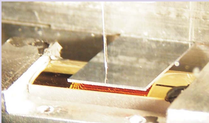
Figure 2. A plane–cylinder geometry is employed in a new Casimir-force experiment under development by Roberto Onofrio and colleagues at Dartmouth College. The plane, a gold-plated silicon wafer 1 cm wide and 200 \mu\text{m} thick, is clamped along one edge between two plates of aluminum and is configured as a mechanical resonator. The vertical white object is an optical fiber used for interferometric distance measurement. In the foreground is the cylinder holder, mounted on a piezoelectric transducer for fine distance control; mechanical actuators provide coarse distance and tilt control. The cylinder, a gold-coated optical-quality cylindrical lens, is 2 cm long and 1 cm wide, with a radius of curvature of 2 cm. A change in the mechanical resonance frequency of the clamped plane will provide a measure of the gradient of the Casimir force. The Dartmouth group hopes to obtain sufficient sensitivity to measure with high accuracy the thermal correction to the Casimir force. (Courtesy of Michael Brown-Hayes and Roberto Onofrio, Dartmouth College.)
