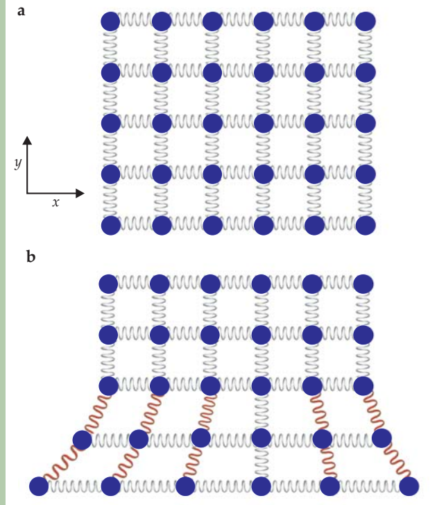
Figure 3. (a) Elastic network in equilibrium with all masses in the reference state. (b) The equilibrium lengths of horizontal springs in successive rows are increased, but vertical springs are not changed. In the configuration shown, the red springs are under tension and are not at their equilibrium lengths. All configurations of the masses in the plane have high energy, so the structure will buckle.
