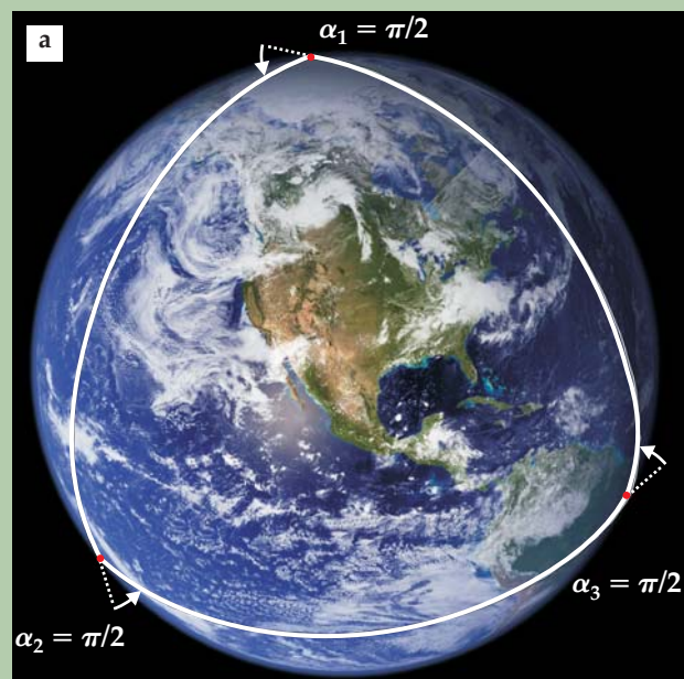
Figure 1. Triangles on spheres have angles that add up to more than \pi radians. (a) In the large triangle, the sum of interior angles is 3\pi/2 radians. (b) The largest triangle on Earth's surface measured by Gauss; the sum of interior angles exceeds \pi by 7.2 \times 10^{-5} radians. (Earth images courtesy of NASA.)
