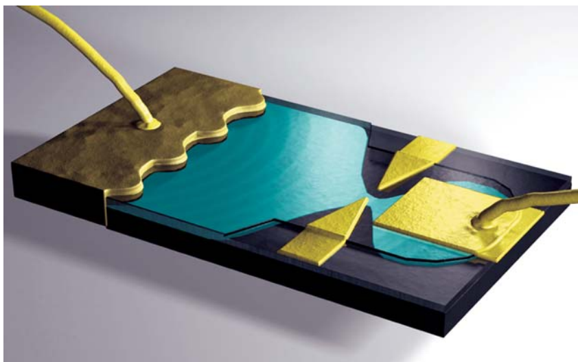
Figure 1. The coherent RC circuit used in the Paris group's experiments is based on a two-dimensional electron gas (blue) that occupies the interface between a layer of gallium arsenide (black) and the layer of aluminum gallium arsenide above it (gray). A pair of pointed, negatively charged surface electrodes pinch the 2DEG to form a quantum point contact. To the right of the QPC is the capacitor, whose plates consist of a quantum dot and a surface electrode. To the left of the QPC is an electrode (brown) that makes ohmic contact with the 2DEG. The wires that sprout from the capacitor's electrode and the ohmic contact connect to the gigahertz power supply and the measuring equipment. (Adapted from ref. 1.)
