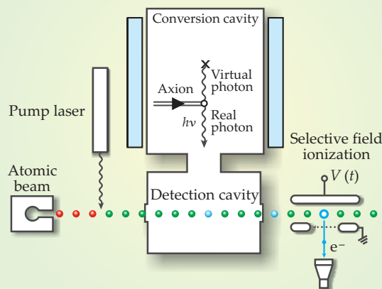
Figure 4. Single-quantum microwave detection. This experimental scheme is used by Seishi Matsuki and colleagues 10 to search for axions. A laser excites a beam of rubidium atoms from the ground state (red) to an |ns\rangle state (green). The beam then traverses the detection cavity, where the spacing between the |np\rangle and |ns\rangle levels is adjusted to equal h\nu , the expected energy of a photon created by an axion's conversion. The coupled atom-cavity system can then efficiently absorb photons. The mixed-population beam that exits the cavity then undergoes selective field ionization, whereby an electron is liberated and detected only from those atoms promoted to the |np\rangle state (blue).
