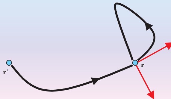
Figure 1. Trajectory of a particle executing bounded motion with energy E . The gradient of the action S(E, \mathbf{r}, \mathbf{r}') , indicated by the red arrows, gives the momentum at point \mathbf{r} . The gradient, however, is multi-valued in general because bound motion loops back on itself. Albert Einstein showed that for certain types of motion the momentum can be expressed as a single-valued vector field on a multiply connected space analogous to the surface of a doughnut.
