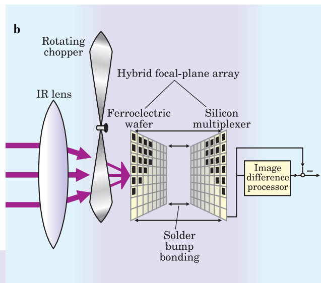
Figure 3. Single- and multiple-element pyroelectric detectors. (a) In this single-element configuration intended to monitor radiation with a wavelength near 10 microns, two lead titanate pyroelectric elements are used. One detector element is exposed to incoming radiation, another shielded under a metal strip. Both crystals are electrically connected with opposite polarities, to cancel out the effect of any drift in ambient temperature. (b) A ferroelectric-hybrid focal-plane device comprises a lens, usually made of germanium to block visible light, and an array of individual ferroelectric elements that are each bonded by tiny balls of solder to elements from a silicon multiplexer. The incident IR radiation must be periodically blocked, here by a chopper, to ensure that a temperature variation is measured. (Adapted from ref. 14 and 15.)
