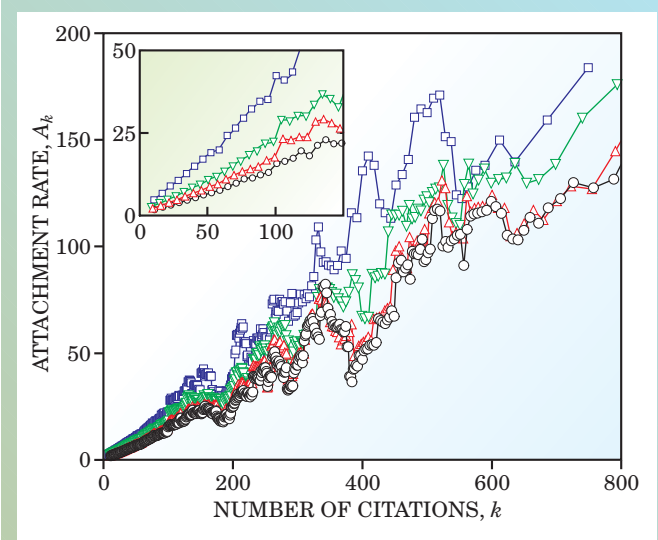
Figure 3. The attachment rate A_k is a nearly linear function of the number of citations k , especially for k less than 150 (inset). The different colors indicate different year ranges for establishing k : 1990–99 (purple), 1980–99 (green), 1970–99 (red), and 1893–1999 (black). The rate A_k is determined from citations in the year 2000. Data have been averaged over a range of \pm 2.5\% . Other time ranges for existing and new citations give similar behavior.
