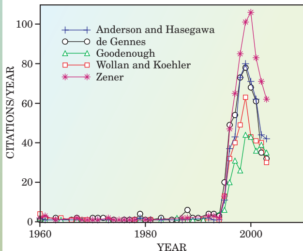
Figure 4. Five revived classics of relevance to colossal magnetoresistance have similar citation histories. Table 2 gives more information about these papers.
