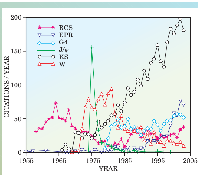
Figure 5. Six classic, highly-cited publications have varied citation histories. The abbreviations are defined in the text.
