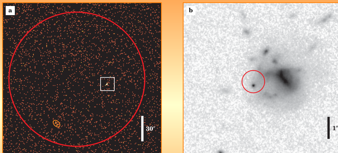
Figure 1. Pinpointing the short gamma-ray burst of 9 July 2005. (a) On the x-ray field image taken three days later by the Chandra orbiter, the red circle indicates the initial localization by the HETE satellite. The bright point source in the box is Chandra 's image of the burst's afterglow. The known x-ray source in the orange oval provides a positional reference. (b) A superposition of optical images from the Hubble Space Telescope in the weeks after the burst pinpoints the afterglow to a fading point source (within the red Chandra localization circle) just inside an irregular spiral galaxy that appears gray. Extended darker areas of the galaxy outside the circle are regions of active star formation. (Adapted from ref. 4.)
