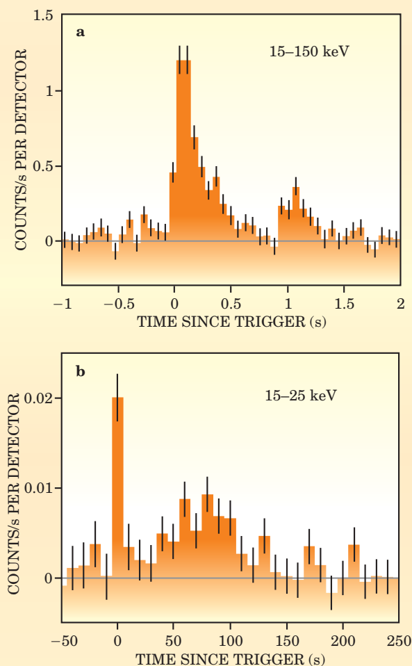
Figure 2. Emission of hard and soft gammas from the short 24 July burst, as recorded by the Burst-Alert Telescope aboard the Swift orbiter. BAT is an imaging array with thousands of detector elements. (a) Within the first two seconds, the record of gammas with energies up to 150 keV shows two prominent short peaks. (b) In addition to those initial peaks, the record of soft gammas (up to 25 keV) detected over the first four minutes shows an additional faint, broad enhancement centered near 80 s. (Adapted from ref. 5.)
