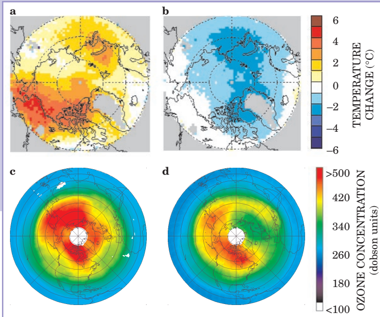
Figure 2. Springtime temperatures in the troposphere (a) warmed on average from the 1980s through the 1990s, especially in the western part of the Arctic, as recorded by the TIROS Operational Vertical Sounder (TOVS). A cooling trend in the stratosphere occurred in springtime during the same period (b). The Total Ozone Mapping Spectrometer measured different ozone levels in the Northern Hemisphere in (c) March 1979 and (d) March 2003. The unit of measure in ozone research is the dobson unit. One DU corresponds to a layer of ozone that would be 0.01 millimeters thick if brought to standard temperature and pressure (0°C and 1 atmosphere). (TOVS images from Overland et al., ref. 4; ozone images from data available at http://toms.gsfc.nasa.gov .)
