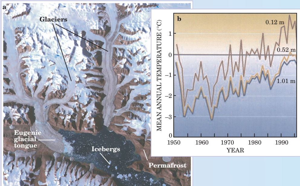
Figure 4. (a) Glaciers on Ellesmere Island and icebergs in Dobbin Bay imaged by the Advanced Spaceborne Thermal Emission and Reflection Radiometer (ASTER) on 31 July 2000. (b) Yearly fluctuations in permafrost temperatures at three sampling depths in Fairbanks, Alaska. (Image courtesy of the University of Alberta, NASA's Goddard Space Flight Center, the US/Japan ASTER Science Team, and the Japan Aerospace Exploration Agency. Permafrost data courtesy of V. Romanosky, University of Alaska, Fairbanks.)
