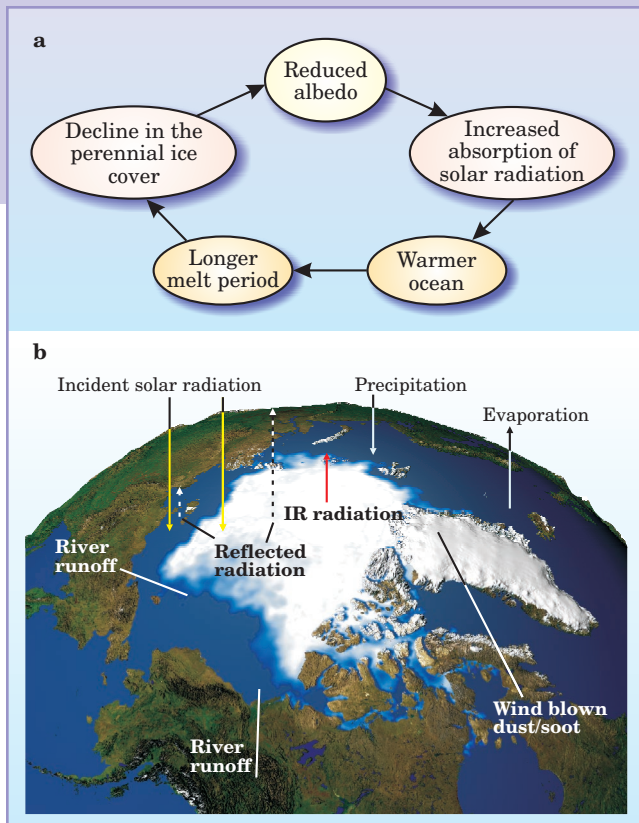
Figure 6. Arctic ice, ocean, and atmosphere are closely interconnected: a change to one influences the others. (a) One possible feedback loop. (b) Some of the key fluxes that affect the Arctic system. The arrows overlay a satellite-derived map of the perennial ice cover when that cover was least extensive in 2002.
