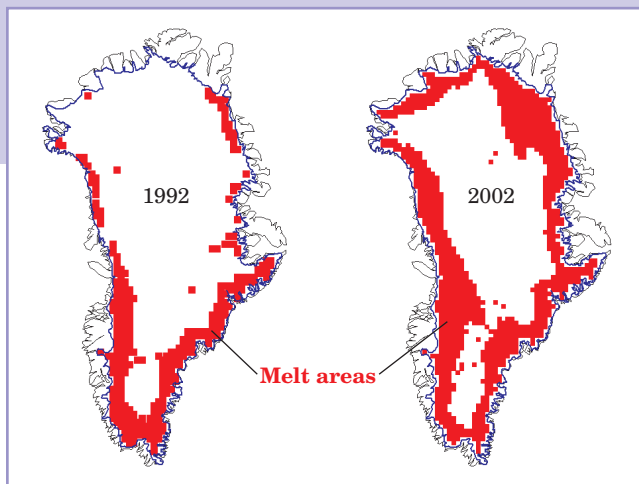
Figure 3. Differences in the expanse of summertime melt over Greenland in 1992 and 2002, illustrated in red. The blue outline delineates the border of the Greenland ice sheet. (Data courtesy of Konrad Steffen and Russell Huff, University of Colorado at Boulder.)
