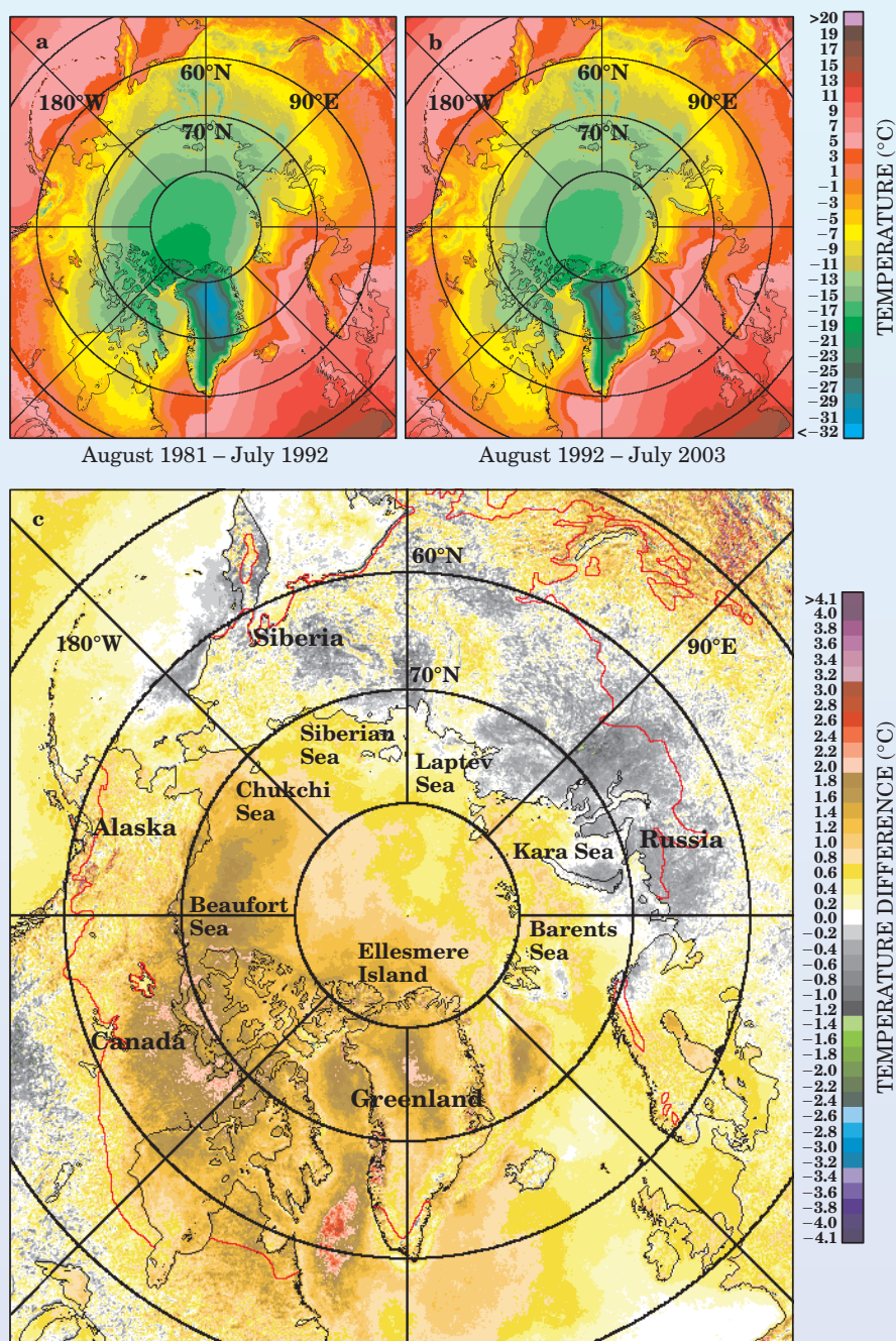
Figure 1. Surface warming is evident from 22 years of IR data collected using the National Oceanic and Atmospheric Administration's series of polar-orbiting satellites: (a) average surface temperature from readings taken between August 1981 and July 1992 and (b) average surface temperature from August 1992 through July 2003. (c) Subtracting the first set of data from the second reveals the net warming trend. The red line represents the southern boundary of the discontinuous permafrost. (Adapted from ref. 2; red-line data courtesy of the United Nations Environment Programme.)
