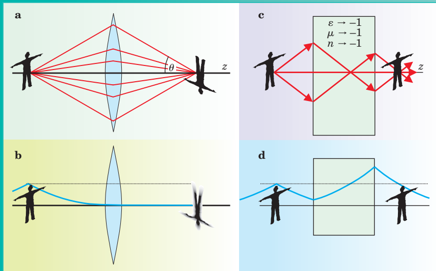
Figure 4. Resolution limitations. (a) For good resolution, conventional lenses need a wide aperture to refract rays at large angles \theta , but even so, they are limited in resolution by the wavelength used. (b) The missing Fourier components of the image are contained in the near field, which decays exponentially (blue curve) and makes negligible contribution to the image. (c) A lens made from a planar slab of negative-index material not only brings rays to a focus but has the capacity (d) to amplify the near field so that it contributes to the image. Such a negative lens thus removes the wavelength limitation. However, the resonant nature of the amplification places severe demands on materials: They must be very low loss.
