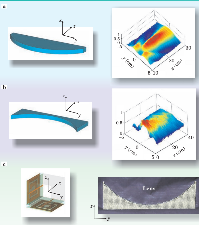
Figure 3. Lightweight, compact lenses can be designed from metamaterials to be relatively free of aberration. (a) A positive-index lens with an index of refraction n of 2.3. On the right is its focusing pattern: Light traveling in the +z -direction is focused at the red peak. Color represents intensity: red, highest; blue, lowest. (b) A metamaterial lens with n = -1 and with the same radius of curvature as in (a), and its focusing pattern. The meta-lens is much lighter than the positive-index lens, a significant advantage for aerospace applications. Although both lenses have the same radius of curvature, the negative lens has a much shorter focal distance. (c) A concave metamaterial lens, designed by Claudio Parazzoli and his colleagues at Boeing Phantom Works, 18 with n \approx -1 at microwave frequencies near 15 GHz. On the left is its unit cell; on the right, a picture of the lens.
