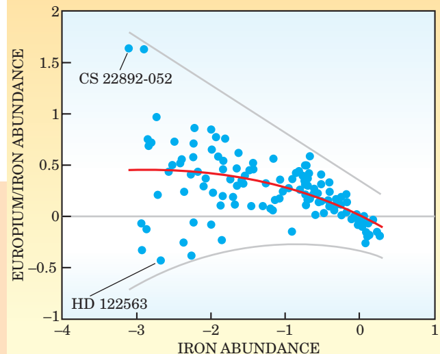
Figure 6. Europium abundance in a large sample of old and young stars, age being inferred from Fe abundance. The halo star HD 122563 is almost as Fe-poor as CS 22892-052, and therefore presumably just about as old, but it has much less Eu, an element made only in the r-process. The red line is a least-square-fit to the data, and the gray flanking curves indicate decreasing scatter in the data with increasing time. Numerical conventions are as in figure 5. Zero on the abscissa means Fe abundance like that of the 4.6-billion-year-old Sun.
