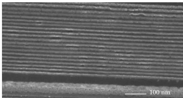
Figure 2. Array of nanowires , each approximately 5 nm in diameter. The lattice constant is about 15 nm. Certain materials parameters important to solid-state devices, such as the average density of dopant atoms, no longer hold meaning at these nanoscale dimensions. At this size scale, however, chemical control over molecular properties is highly developed.
