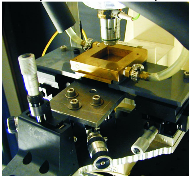
The experimental setup. The gold-colored tray houses the plastic container for the DNA solution. Above it is the microscope objective for imaging the progress of the trapping. (Courtesy of Dieter Braun.)
