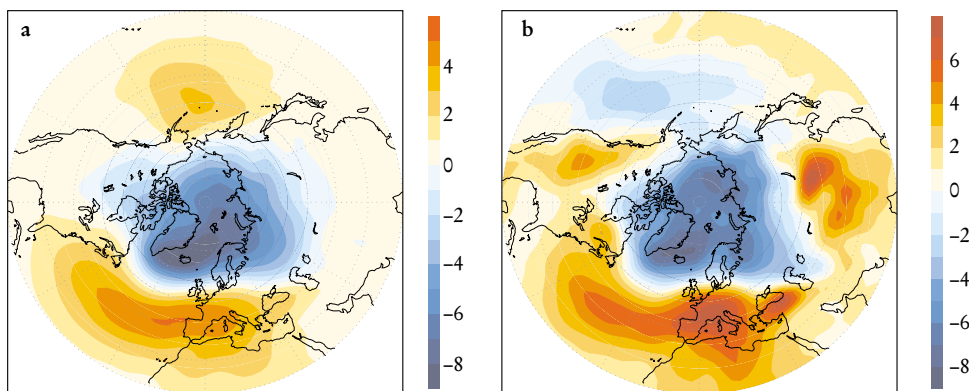
FIGURE 1. THE 30-YEAR TREND in sea-level atmospheric pressure resembles the Northern Hemisphere annular mode (NAM). (a) The NAM is a recurrent pattern in the deviation of sea-level pressures from their long-term averages. The figure shows the NAM on a typical high-index day, displaying relatively low pressures over the polar cap and relatively high pressures at mid latitudes. The color bar gives pressure in units of hectopascals (1 atmosphere = 1013 hPa). (b) The rate of change of sea-level pressure with time based on data collected from January to March over the 30-year period, 1968–97. The numbers on the color bar are in units of hPa/(30 yr), and so one may think of the figure as giving the change in sea-level pressures over the cited 30-year period. The change in the pressure field is remarkably similar to the NAM illustrated in the left panel. (Adapted from ref. 9.)
