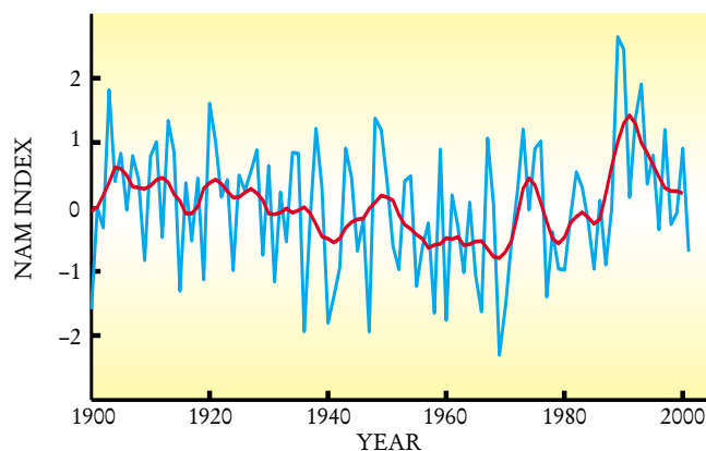
FIGURE 6. WINTERTIME INDICES of the Northern Hemisphere annular mode during the past 100 years, given in terms of standard deviations from the 100-year mean. The blue line shows January–March averages while the red line displays a five-year running average. Note that the NAM indices have significantly risen since the mid-1960s, but have fallen off somewhat in more recent years. (Adapted from ref. 9.)
