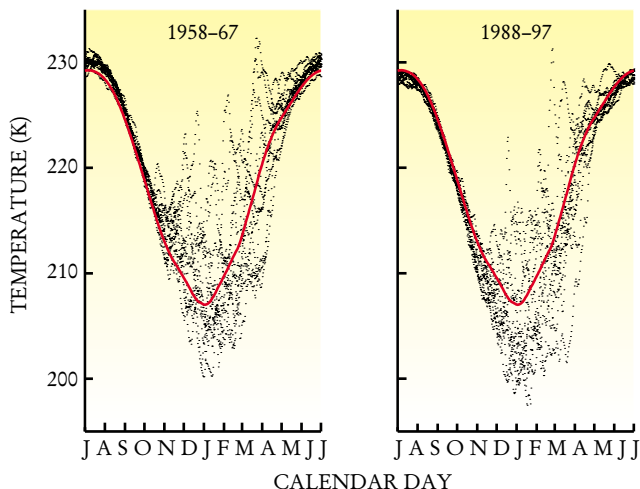
FIGURE 5. TEMPERATURE AT 20 KM over the Northern Hemisphere polar region as a function of calendar day. The horizontal axis runs from July to July. The graph in the left panel shows data for the decade 1958-67. Its companion gives data for the later decade 1988-97. The points on the scatter plots indicate daily measurements, while the solid lines give the average over the 40-year period 1958-97.
