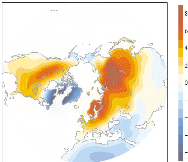
FIGURE 3. AIR TEMPERATURES are warmer over much of the Northern Hemisphere on high-index days (as defined in the text) of the Northern Hemisphere annular mode. The map shows the difference (in ^{\circ}\text{C} ) between mean surface air temperatures on low-index NAM days and those on high-index days. (Adapted from ref. 2.)
