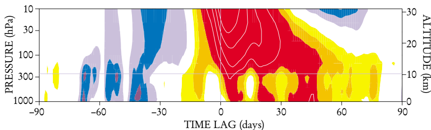
FIGURE 4. TIME-HEIGHT DEVELOPMENT of the strength of the westerlies in the 55\text{--}65^{\circ}\text{N} latitude belt for 18 events, during the past 40 winters, in which the intensity of the polar night jet at the 30-km level (along the top of the diagram) dropped below a specified threshold value. Time lag in the figure is relative to the dates on which those 18 events occurred. The color shading and contours indicate the intensity of the westerlies: Blue shades denote stronger than normal intensities and warm colors denote weaker intensities than normal. The thin horizontal line indicates the base of the stratosphere. (Adapted from ref. 5.)
