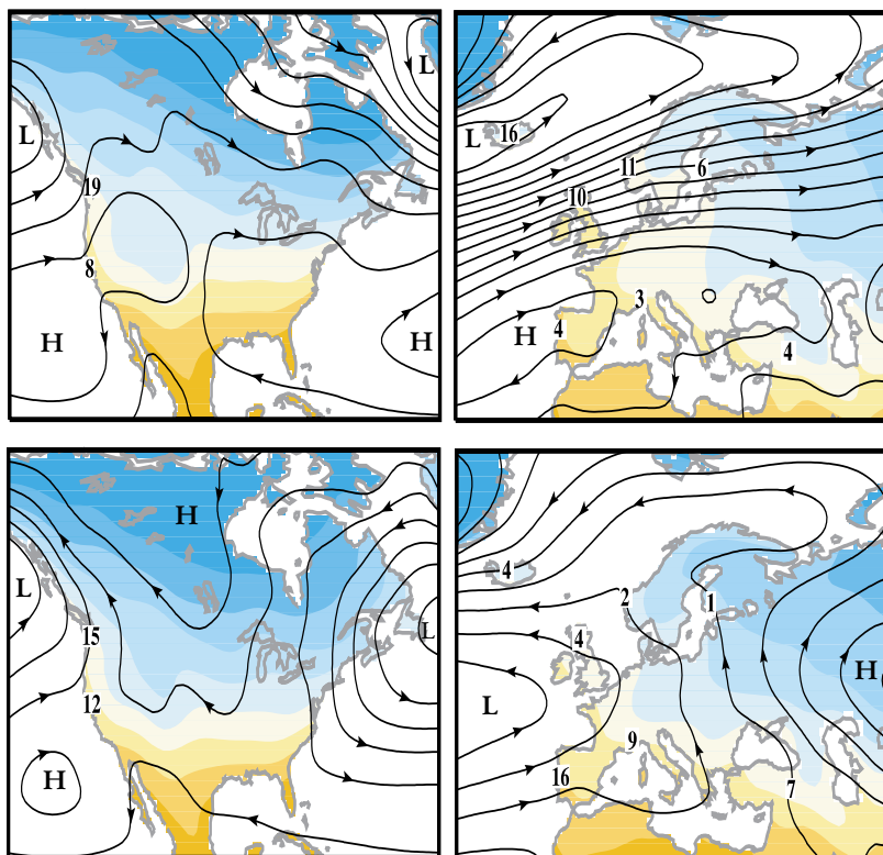
FIGURE 2. COMPOSITE MAPS of surface air temperature (shading), sea-level pressure (contours) and precipitation (the numbers indicate cm/month) for (top) high Northern Hemisphere annular mode-index days, as defined in the text, and (bottom) low NAM-index days. The maps are based on data collected from January to March over the 40-year period, 1958–1997. Contour intervals are 5°C for temperature (blue shades indicate temperatures below 0°C) and 3 hectopascals for sea-level pressure. (Adapted from ref. 2.)
