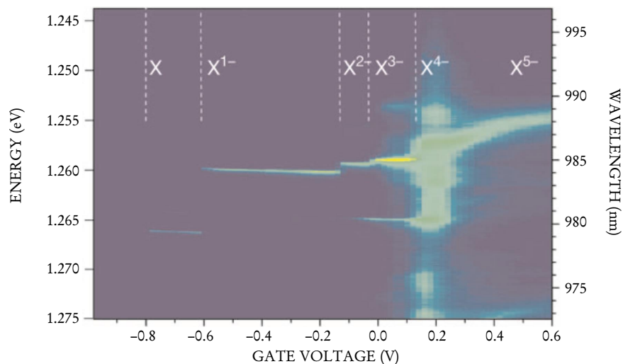
FIGURE 4. INCREASING THE GATE voltage injects electrons, one by one, into a charged quantum dot. As a result, the QD's photoluminescence spectrum changes. Here, dark blue, green, and yellow correspond to low, medium, and high photoluminescence, respectively. The laser power is low enough that only a single exciton exists at a time in the QD. The exciton recombines and emits the luminescence whose spectrum contains information about the charge state of the QD. When four electrons are inside the QD, tunneling out of the QD becomes so fast that the spectral lines broaden dramatically. (Adapted from ref. 15.)
