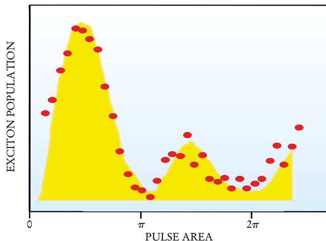
FIGURE 5. RABI FLOPPING DEMONSTRATES the coherent control of the exciton's wavefunction. In this differential transmission experiment, a single pump pulse excites the quantum dot with increasing intensity, while a second, probe pulse measures the change in transmission. This differential transmission is proportional to the difference in the probabilities of the QD's being in the ground or excited state. The transmission goes through a Rabi oscillation as the pump (with a 2\pi pulse) drives the QD up to the exciton state and then back down to the ground state. The oscillation amplitude likely decays with increasing laser power because of the excitation of additional electrons nearby that create additional dephasing.
