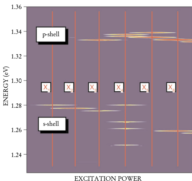
FIGURE 3. THE PHOTOLUMINESCENCE SPECTRUM from a single \text{In}_{0.60}\text{Ga}_{0.40}\text{As} quantum dot changes as the laser excitation power increases. Bright regions indicate strong emission intensities; blue regions indicate low intensities. At low power, a single exciton transition ( X_1 ) is observed. As the power is increased, multiexciton states emerge. The biexciton ( X_2 ) is formed out of two excitons in the s state and has one doubly degenerate transition. However, triexcitons ( X_3 ) and higher multiexcitons also contain at least one exciton derived from the p state. (Adapted from ref. 4.)
