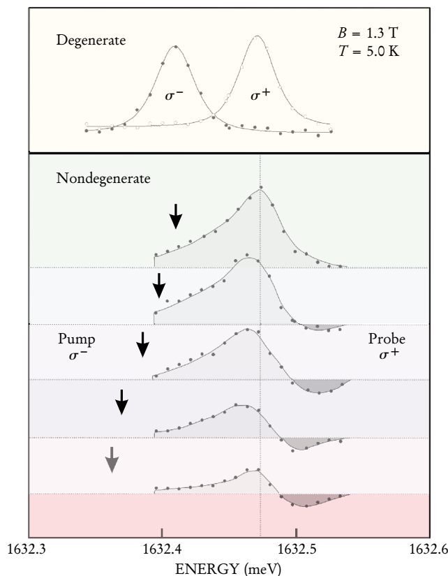
FIGURE 6. A SINGLE QUANTUM DOT can be put into a quantum superposition state by using a pair of mutually coherent lasers. The top panel shows the two degenerate states of the system, denoted by their resonances, \sigma^\pm . The bottom panels show what happens when the system is pumped by a laser tuned to the \sigma^- resonance (the arrows indicate the precise energy) and probed with a laser tuned to the \sigma^+ resonance. Without entanglement, the lineshape would simply decrease in amplitude as the pump laser moved further off resonance. However, the two states are entangled through Coulomb interactions, as evidenced by the negative contribution to the lineshape. Subsequent measurement of the state of one of the excitons (that is, determining whether it is present or not) determines the state of the other (that is, if one is present, the other must be absent). (Adapted from ref. 16.)
