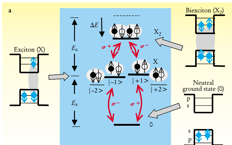
FIGURE 2. THE ELEMENTARY OPTICAL excitation of a quantum dot is the exciton (denoted by X). (a) In QDs with disklike symmetry, the lowest energy exciton has four substates arising from spin. Two of these exciton substates normally have angular momentum values of \pm 1 and have optically allowed transitions \sigma^\pm to the QD's ground state (denoted by 0). The other two exciton substates are normally inaccessible and have angular momentum projections of \pm 2 . A second exciton puts the QD into a biexciton state ( X_2 ), which has an energy reduced slightly ( \Delta E ) by Coulomb interactions among the particles. (b) A charged exciton in a QD with a single electron has a spin-1/2 ground state that has two spin substates. An exciton excited in the presence of this extra electron contains three particles and is sometimes called a trion ( X^- ). The lowest-energy trion has two substates arising from the two possible hole states (the two electrons form a spin singlet).
