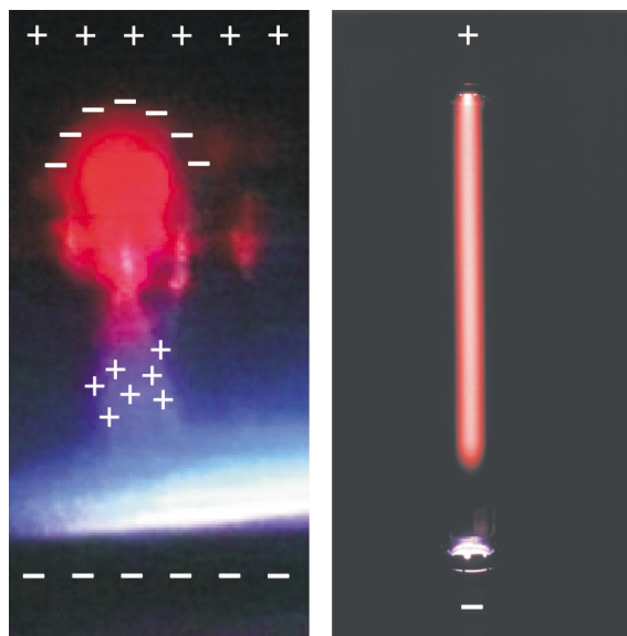
FIGURE 3. SPRITE LIGHT in the atmosphere (left) and in a laboratory glow discharge tube (right). In both cases, the light near the positive (anode) end is red and arises from the collisional excitation of neutral nitrogen molecules by free electrons. Also in both cases, the light near the negative (cathode) end is blue and arises from the collisional excitation of N_2^+ ions by free electrons.
