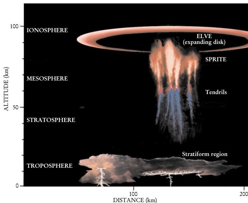
FIGURE 1. SPRITES AND ELVES are triggered by the positive cloud-to-ground lightning flashes that occur in the stratiform regions of mesoscale convective systems. (Adapted from W. A. Lyons, R. A. Armstrong, E. A. Bering III, E. R. Williams, EOS , volume 81, page 373, 2000.)
