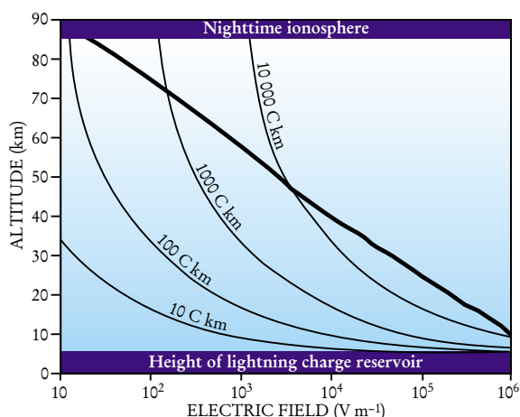
FIGURE 2. PHYSICAL CONDITIONS between conductive Earth and conductive ionosphere necessary for dielectric breakdown and the initiation of sprites, as predicted by C. T. R. Wilson. The bold curve represents the density-dependent dielectric strength of air, while the curved lines represent the electric field strength imposed by lightning for various values of lightning charge moment.
