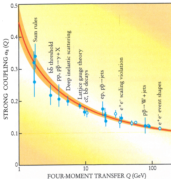
FIGURE 4. THE RUNNING COUPLING “CONSTANT” \alpha_s for the strong interaction is predicted by QCD to decrease with increasing energy and momentum. That’s asymptotic freedom. The red curve is the predicted dependence of \alpha_s on Q , the magnitude of the four-momentum transfer at a QCD vertex. An empirical input is the measured coupling of a quark pair to a virtual gluon at the Z boson mass; the orange swath reflects its uncertainty. The theory yields excellent agreement with a great variety of experiments, 14 shown by the data points and labels. The open points are results based on the general shapes of many-particle final states in momentum space.
