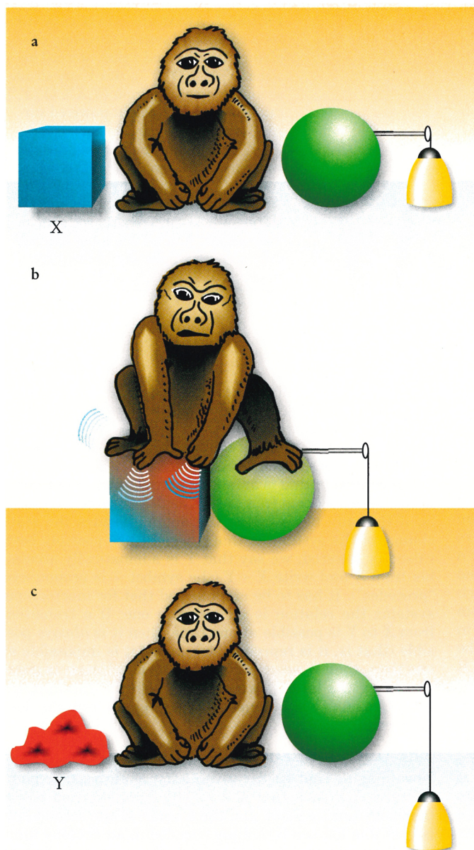
FIGURE 1. THE SECOND LAW OF THERMODYNAMICS says that increased entropy characterizes those final states of a macroscopic system that can be reached from a given initial state without leaving an imprint on the rest of the universe, apart from the displacement of a weight. The scenario shown here illustrates that the process can be quite violent. (a) A system in an equilibrium state X (blue) is placed in a room with a gorilla, some intricate machinery (green), and a weight. (b) The gorilla, machinery, and system interact and the system undergoes a violent transition. (c) The system is found in a new equilibrium state Y (red), the gorilla and machinery are found in their original state, while the weight may have been displaced. The role of the weight is to supply energy (via the machinery) both for the actions of the gorilla and for bringing the machinery and gorilla back to their initial states. The recovery process may involve additional interactions between machinery, system, and gorilla—interactions besides those indicated in (b).
