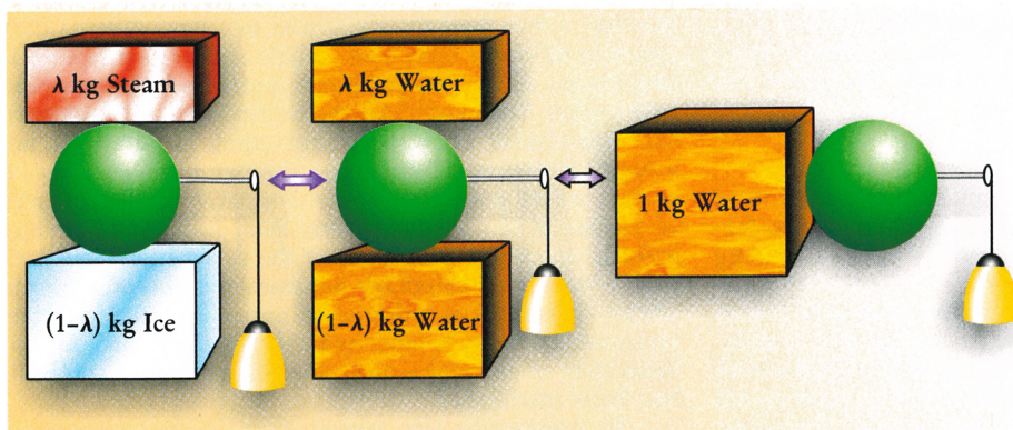
FIGURE 3. DEFINITION OF ENTROPY. One can define the entropy of 1 kg of water in a given state (represented by the orange color) by obtaining the state from a fraction \lambda kg of steam in a fixed, standard state (red) and a fraction 1 - \lambda kg of ice in a fixed, standard state (blue), with the aid of a device (green) and a weight (yellow). The device returns to its initial state at the end of the process, but the weight may end up raised or lowered. The entropy S_{\text{water}} , measured in units of S_{\text{steam}} , is the maximum fraction \lambda = \lambda_{\text{max}} for which the transformation to 1 kg of water in the given (orange) state is possible. The system of steam and ice is used here only for illustration. The definition of entropy need not involve phase changes.
