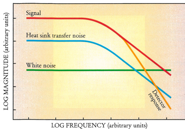
FIGURE 3. AN INSTANTANEOUS DEPOSITION of energy into a calorimeter produces a signal pulse that decays exponentially with time constant \tau . In the frequency domain, shown here, the signal (red) is roughly constant until f \approx 1/2\pi\tau , after which it falls off as 1/f . The noise due to the random transfer of energy across the link to the heat sink (blue) has the same frequency distribution as the signal. If this so-called phonon noise were the only source of noise, the signal-to-noise ratio would be frequency independent, and the measurement error could be made arbitrarily small by employing a sufficiently large bandwidth. In reality, a frequency-independent noise term (green) and the effect of a finite detector response time (orange extension from red line) reduce the signal-to-noise ratio at high frequencies, effectively limiting the usable bandwidth.
