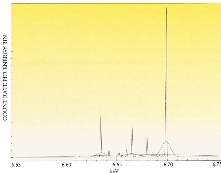
FIGURE 1. IRON K EMISSION LINES from a model plasma at 7 \times 10^7 K, as viewed with a spectral resolution of 1 (blue), 10 (green), and 100 eV (red). Clearly, high-resolution detectors must be used to exploit the full diagnostic potential of x-ray spectroscopy.
