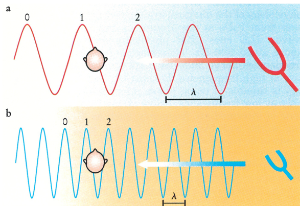
FIGURE 3. INTERAURAL TIME DIFFERENCES , given by the difference in arrival times of waveform features at the two ears, are useful localization cues only for long wavelengths. In (a), the signal comes from the right, and waveform features such as the peak numbered 1 arrive at the right ear before arriving at the left. Because the wavelength is greater than twice the head diameter, no confusion is caused by other peaks of the waveform, such as peaks 0 or 2. In (b), the signal again comes from the right, but the wavelength is shorter than twice the head diameter. As a result, every feature of cycle 2 arriving at the right ear is immediately preceded by a corresponding feature from cycle 1 at the left ear. The listener naturally concludes that the source is on the left, contrary to fact.
