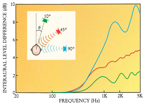
FIGURE 2. INTERAURAL LEVEL DIFFERENCES , calculated for a source in the azimuthal plane defined by the two ears and the nose. The source radiates frequency f and is located at an azimuth \theta of 10^\circ (green curve), 45^\circ (red), or 90^\circ (blue) with respect to the listener's forward direction. The calculations assume that the ears are at opposite poles of a rigid sphere.
