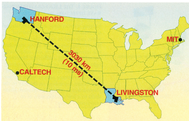
FIGURE 2. THE TWO LIGO SITES, 3030 km apart, in Hanford, Washington and Livingston, Louisiana, will work in coincidence. The recent photo of the Hanford site shows the two orthogonal 4 km vacuum pipes going off into the distance. The vacuum system also houses a smaller auxiliary interferometer, with 2 km arms to help distinguish true gravitational wave signals from noise.
