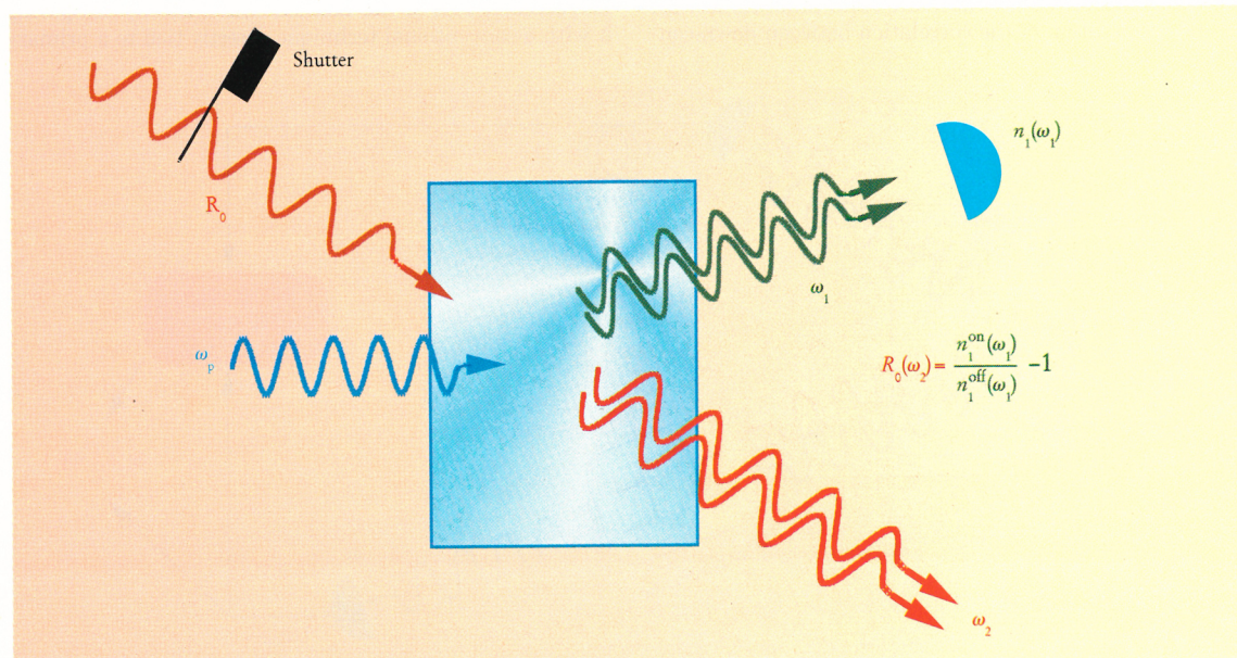
FIGURE 5. SPECTRAL RADIANCE of the photon beam R_0 can be measured at \omega_2 by overlapping it with the crystal along the \omega_2 output direction. The double wavy lines at output frequencies \omega_1 and \omega_2 indicate the enhancement of photon-pair production caused by adding the R_0 input. Energy conservation dictates that \omega_1 + \omega_2 = \omega_p . If one measures the n_1(\omega_1) signal with an uncalibrated detector in a convenient visible region, one can get the absolute radiance of R_0 in the more difficult infrared region \omega_2 simply from the ratio of the visible detector signals with R_0 on and off.
