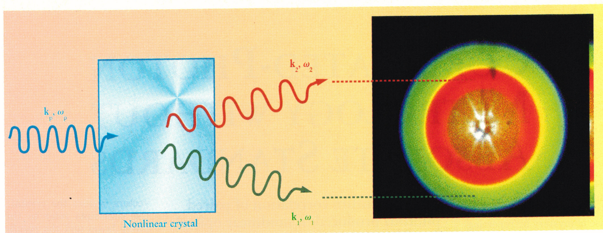
FIGURE 1. PARAMETRIC DOWN-CONVERSION, turning a single photon entering an optically nonlinear crystal into two photons coming out, is essentially the inverse of sum-frequency generation. The energy \hbar\omega and momentum \hbar\mathbf{k} of the incident photon equals the sums of the outgoing energies and momenta. The concentric circles of output light in different colors (at right), azimuthally symmetric about the monochromatic pump-beam axis, indicate the broad spectral range of the down-converted light. At their center, one sees some of the pump light leaking around a beam stop.
