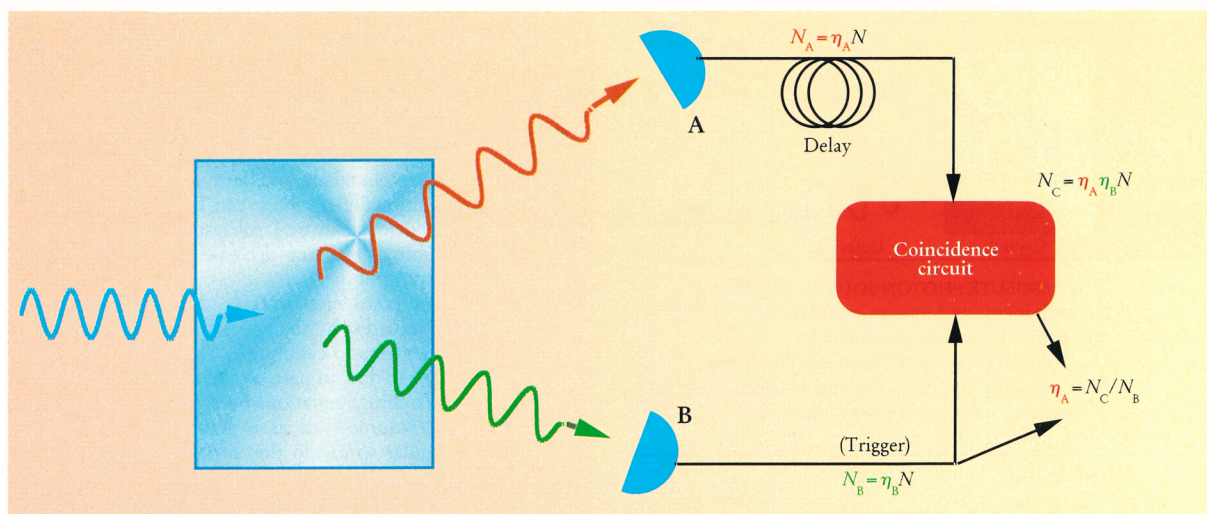
FIGURE 2. ABSOLUTE QUANTUM-EFFICIENCY DETERMINATION. N is the true number of correlated photon pairs produced in the down-conversion crystal, and N_A and N_B are the tallies of photons recorded individually by detectors A and B, with respective unknown efficiencies \eta_A and \eta_B . The number of expected coincidence counts N_C being N times the product of these two efficiencies, one arrives at the efficiency of A, the detector to be calibrated, without having to know the efficiency of B, the trigger detector.
