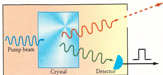
FIGURE 4. NEW ABSOLUTE PHOTON SOURCE exploits the constraints of simultaneity and energy-momentum conservation on pairs of photons produced by down-conversion of pump-beam photons in a nonlinear crystal to specify not only the direction and wavelength of an output photon, but also its time of emission, simply by recording its partner in a detector.
