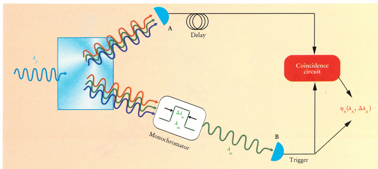
FIGURE 3. WAVELENGTH DEPENDENCE of the efficiency \eta_A(\lambda_A, \Delta\lambda_A) of A, the detector to be calibrated, can be determined with the spectral filtering optics confined to the optical channel of B, the trigger detector. So it is not necessary to know the transmittance of the spectrally selective element. The frequency \omega_A = 2\pi c/\lambda_A is given by \omega_p , the pump-beam frequency minus \omega_m , the center of the monochromator's passband \Delta\lambda_m .
