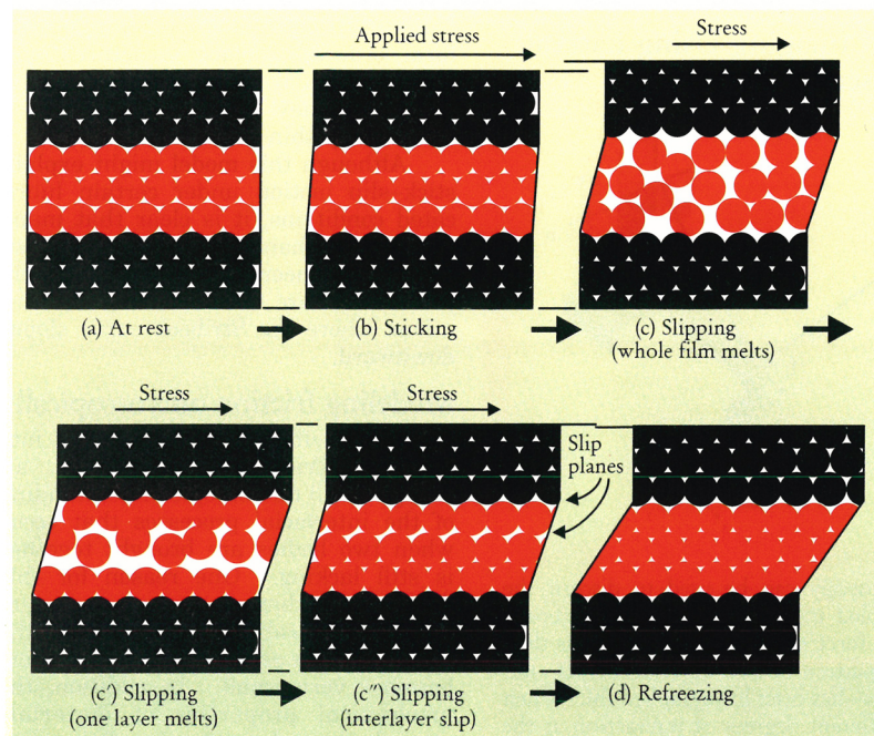
FIGURE 4. MOLECULAR REARRANGEMENTS occurring in a molecularly thin film of simple chain molecules between two solid surfaces during shear. (From ref. 13.)
