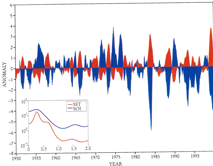
FIGURE 1. COVARYING ATMOSPHERIC AND OCEANIC INDICES. Plotted in red are anomalies (departures from the long-term mean) of sea surface temperature (SST), averaged over the east-central Pacific at the equator for 1950–97. Plotted in blue is the SOI (Southern Oscillation Index), which consists of normalized surface pressure difference between Tahiti, in the mid-Pacific, and Darwin, Australia. The SOI provides a measure of the pressure gradient across the tropical Pacific, and that gradient, in turn, is related to equatorial wind variations. During negative phases of the SOI, the anomalous winds blow eastward from high to low pressure along the equator. The SOI is normalized by the standard deviation, while SST is in degrees C. Power spectra of these time series (inset) exhibit a broad but robust peak centered at approximately four-year period (axis in cycles per year). A smaller (and less statistically robust) peak near two-year period is sometimes noted but is not resolved here.
