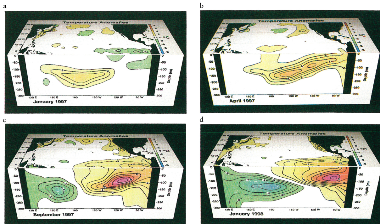
FIGURE 2. THE TRANSITION INTO THE 1997–98 EL NIÑO WARM PHASE, showing evolution of anomalies in sea surface temperatures and subsurface temperatures along the equator. In January 1997 (a), the surface temperature in the east was colder than normal, but in the west, the warm subsurface temperature anomalies associated with a lower thermocline had existed for some time, partly due to the movement of warm water from the equator. Because the pressure gradients associated with these anomalies were not in balance with the wind stress, they evolved in time, spreading eastward along the equator. By April 1997 (b), the thermocline had deepened in the east, but the effects of subsurface warm anomalies were not seen in surface temperatures. By September 1997 (c), the warm anomalies had been communicated to the surface and had set in motion the atmospheric feedback described under the Bjerknes hypothesis. In response to weakened easterly winds, the thermocline slope reduced further, intensifying warm anomalies in the east. In the west, the shallowing of the thermocline produced cold anomalies, which are customarily stronger off the equator. By January 1998 (d), this process had produced large anomalies both at and below the surface in the east. The slower adjustment process involving off-equator anomalies in the west produced growing subsurface cold anomalies. Now, in late 1998, the subsequent eastward extension of these anomalies is swinging the system into the predicted cold phase of the cycle. Known as La Niña, this phase develops much like the anomalies shown for El Niño, but with opposite sign. (Figure courtesy of David Pierce, Scripps Institute of Oceanography.)
