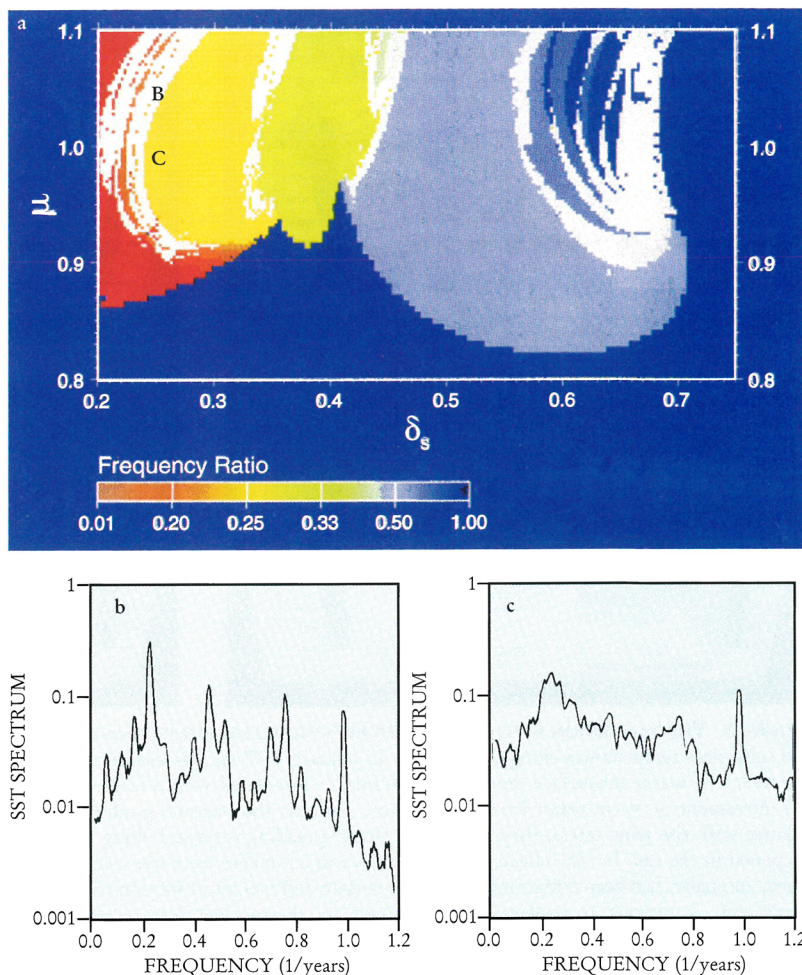
FIGURE 3. DEPENDENCE OF CHAOTIC OR FREQUENCY-LOCKED BEHAVIOR on model parameters for an El Niño model from which weather noise has been excluded. a: The vertical axis is a coupling parameter, which affects the amplitude of the simulated El Niño through the strength of atmospheric wind anomalies. The horizontal axis is a surface-layer parameter, inversely related to the strength of momentum mixing between the surface layer and the layer below. The surface-layer parameter affects the length of the simulated cycle, since stronger currents tend to change surface temperature faster. The plot represents the result of about 3000 500-year simulations, with each simulation classified as chaotic (gray) or frequency locked (color). In the frequency-locked case, color represents the frequency ratio of the El Niño oscillation to that of the annual cycle. For example, 0.33 is one El Niño every 3 years, while 0.30 is three El Niños every 10 years. Ratios of integers occur only for frequency-locked solutions. By contrast, the chaotic solutions occur between the strongly frequency locked regions, where the solution tends to lock first on one interval and then on the other. Chaotic solutions yield power spectra that still have spectral peaks, but a broadband background typical of chaotic solutions. b: the power spectrum for point B in a . c: the power spectrum from the point marked C in a , but with a representation of weather noise included. It exhibits the broadening of the four-year peak that is comparable to more complex models and to observations (see figure 1). (Adapted from Jin et al. , Physica D 98 , 442, 1996.)
