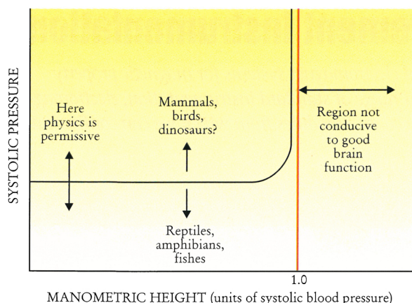
FIGURE 5. SYSTOLIC BLOOD PRESSURE as a function of animal height. The pressure shows little regular variation among small- and medium-sized mammals. But it must (and does) rise in large mammals so that it remains at least as great as manometric height (the product of blood density, gravitational field strength and the animal's height).
