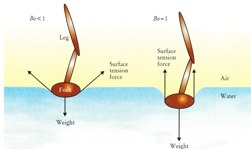
FIGURE 3. WALKING ON WATER. The schematic diagram shows legs pressing on the air–water interface where surface tension is more than adequate for support (Bond number Bo < 1 ), and where the weight of the animal just reaches the force that can be sustained by surface tension ( Bo = 1 ).
