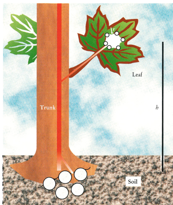
FIGURE 4. CONTINUOUS COLUMNS OF LIQUID SAP, nearly pure water, run up a tree and connect the water between soil particles with the wet walls of the cells within the leaves that contact the air. Supporting the columns of height h , as well as offsetting the pressure losses due to flow and capillary forces within the soil, requires that the radius of curvature r of the final air–water interfaces be very small.
