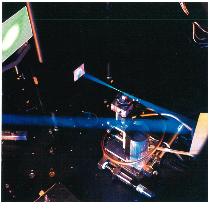
FIGURE 1. ULTRAINTENSE PULSE of laser light comes to a focus, where it interacts with a 1 mm wide jet of helium gas propagating upward, producing a high-energy, collimated beam of electrons with energies up to 50 MeV. The electrons light up the phosphor screen at the upper left. Aluminum foil, which appears pink in this photo, blocks the laser light.
