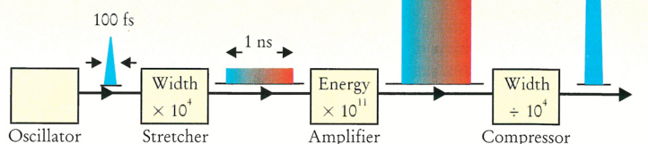
FIGURE 3. CHIRPED PULSE AMPLIFICATION. a: The CPA concept. An oscillator produces a short pulse, which is then stretched by a factor of 10^3 to 10^5 , from the femtosecond to the nanosecond regime, reducing its intensity accordingly. The intensity is now low enough that the pulse can be amplified and the stored energy can be safely extracted from the amplifier without fear of beam distortions and damage. After extraction, the pulse is recompressed, ideally to its initial width. b: The matched stretcher and compressor. The stretcher (top) is composed of a telescope of magnification 1 between two antiparallel diffraction gratings. Note that in this configuration the red wavelengths have a shorter path than the blue ones. Conversely, the compressor (bottom) is composed of a pair of parallel gratings in which the optical length for the blue is shorter than that for the red. The gratings are matched over all orders.
