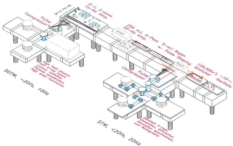
FIGURE 4. AMPLIFICATION CHAIN. The schematic represents a tabletop titanium:sapphire chirped pulse amplification system at the University of California, San Diego, that can produce 5 TW and 50 TW laser pulses.
