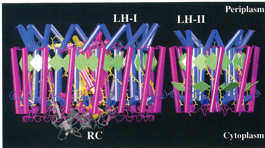
FIGURE 2. THE MODELED PHOTOSYNTHETIC UNIT showing the arrangement of its main pigment-protein complexes—namely, LH-II, LH-I and the photosynthetic reaction center (RC). The unit has been constructed using the model structure of the Rb. sphaeroides LH-I 8 and the crystal structures of the Rb. sphaeroides RC and Rs. molischianum LH-II. 7 We note that recent electron microscopy data suggest that the LH-II of Rb. sphaeroides contains 9 \alpha\beta -heterodimers instead of 8 as in the LH-II of Rs. molischianum . The \alpha -helices are represented as cylinders with the \alpha -apoproteins of both LH-I and LH-II shown in blue and the \beta -apoproteins in magenta, respectively. The RC is a complex of three protein subunits shown in different colors. The pigment molecules—that is, the BChls and carotenoids—are shown in green and yellow, respectively. The figure is actually to scale, with the relative positions of LH-I and LH-II being derived by optimizing the LH-II's interaction with LH-I.
