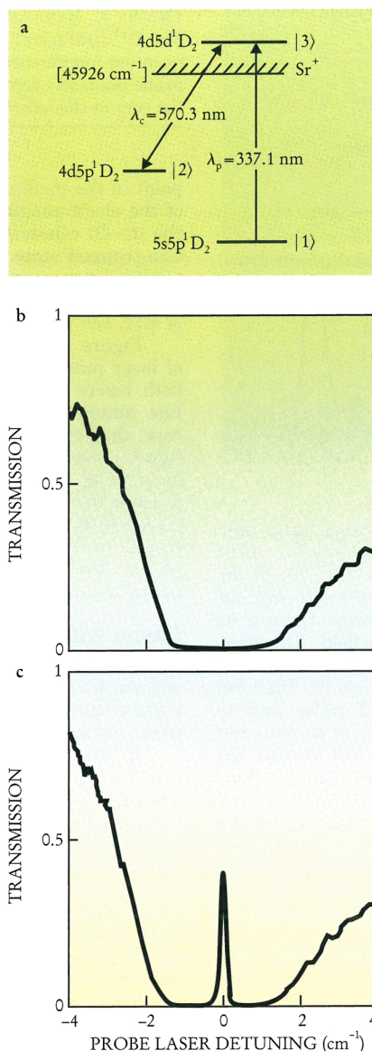
FIGURE 3. ELECTROMAGNETICALLY INDUCED TRANSPARENCY IN STRONTIUM VAPOR. 1 a: Partial energy-level schematic. The frequency of a laser of wavelength \lambda_c is held fixed. Because this laser couples states |2\rangle and |3\rangle , it is termed the coupling laser. The frequency of a probing laser of wavelength \lambda_p is varied. b: Transmission versus probe laser detuning with the coupling laser absent. The minimum transmission in this figure is \exp(-20) . c: Transmission versus probe laser frequency with the coupling laser present. The ratio of the transmitted to the incident light is now about 40%. Under the conditions of this experiment, almost all of the atoms remain in the ground state |1\rangle .
