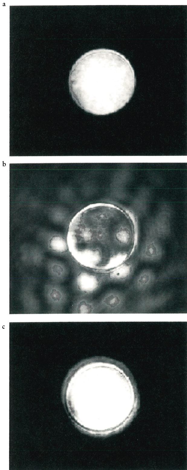
FIGURE 1. ELIMINATION OF OPTICAL SELF-FOCUSING in lead vapor through electromagnetically induced transparency.
