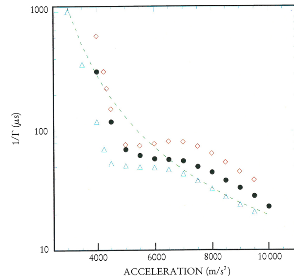
FIGURE 5. TUNNELING LIFETIME as a function of acceleration. The experimental data are marked by solid dots.
