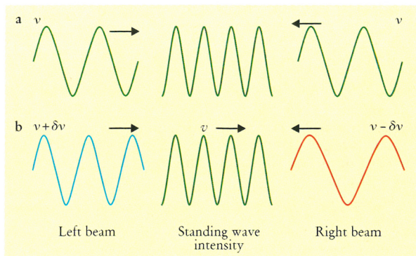
FIGURE 2. LASER BEAM CONFIGURATIONS to produce a standing wave that is (a) stationary or (b) moving to the right with velocity v = \lambda \delta \nu in the laboratory frame. An accelerating standing wave is produced by increasing the frequency difference 2\delta \nu linearly in time. In the Texas experiments, for example, a linear ramp of 4 MHz in 800 \mu s created a potential accelerating at 1500 m/s 2 .
