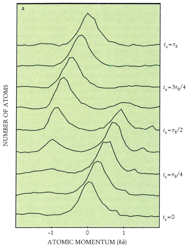
FIGURE 3. BLOCH OSCILLATIONS OF ATOMS in the fundamental band. a: Momentum distribution of atoms in the accelerated frame for acceleration times t_a ranging from 0 to the Bloch period, \tau_B = 8.2 ms. Bragg reflection of the matter wave occurs when the atomic momentum p approaches the Bragg condition, p = \hbar k . (The small peak in the right wing of the first five spectra is an artifact created by a stray reflection of the Raman beams on the cell windows). b: Measured mean atomic velocities (circles) in units of the photon recoil velocity v_R compared to theory (solid line). Both sets of data are for a light potential depth U_0 = 2.3 E_R and acceleration a = -0.85 m/s 2 . (From ref. 6.)
