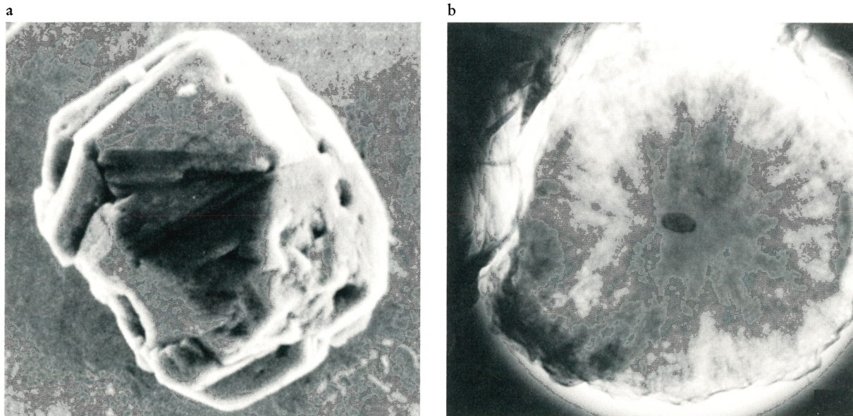
FIGURE 1. STARDUST IN THE LABORATORY , as evident in electron micrographs. a: A presolar silicon carbide crystal from the Murchison meteorite. The ^{12}\text{C} / ^{13}\text{C} ratio of this crystal is 39—radically different from the solar value of 89, which tags it as a grain that originated outside the Solar System. This crystal most likely condensed in the expanding atmosphere of a star on the asymptotic giant branch. It measures about 4\ \mu\text{m} across. (Photo courtesy of Sachiko Amari.) b: A 70 nm thick section of a presolar graphite spherule. The crystal in the center of the spherule is titanium carbide, a refractory mineral that formed before the graphite and served as a nucleation center for its growth. The dark, radial spokes in the image are an electron diffraction effect; in reality, the graphite layers are concentric.
