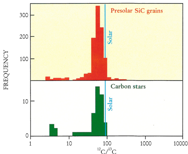
FIGURE 3. COMPARING THE DISTRIBUTION of ^{12}\text{C} / ^{13}\text{C} ratios among presolar silicon carbide grains with astronomical values measured by David Lambert and coworkers for carbon stars using spectroscopic methods. The figure illustrates two important findings. First, most of the presolar SiC grains and carbon stars measured do not have the same ^{12}\text{C} / ^{13}\text{C} ratio as the Sun. Second, the similarity of the two distributions demonstrates that the carbon in presolar grains came originally from many presolar carbon stars.
