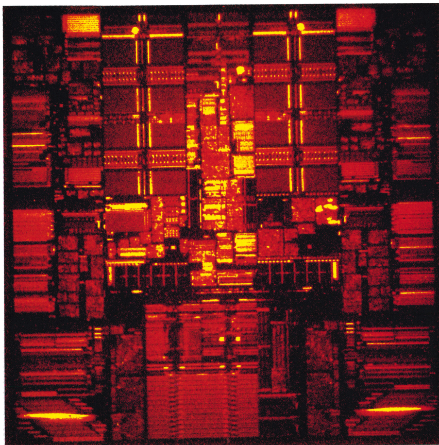
FIGURE 1. A MODERN MICROPROCESSOR —in this case, the chip used in IBM S/390 mainframes—based on the complementary metal oxide semiconductor field-effect transistor (CMOSFET) technology. Measuring 18 mm on a side, the chip contains over eight million transistors and has features as small as 0.3 \mu\text{m} . This image, which was taken in the near infrared by a cooled charge-coupled device camera, shows the weak light emitted by the chip when individual CMOSFET gates switch on and off. Charge carriers passing through the channels of modern CMOSFET gates experience electric fields of over 10^7 \text{ V cm}^{-1} and can acquire appreciable kinetic energy, some of which is converted to light energy. The particular circuit activity shown in this image is due to the clocks in the chip, and to a signal propagating through a chain of 64 000 latches in the circuit. (Figure made by Jeffrey Kash and James Tsang at IBM's Thomas J. Watson Research Center; originally published in Science , vol. 276, p. 1987.)
