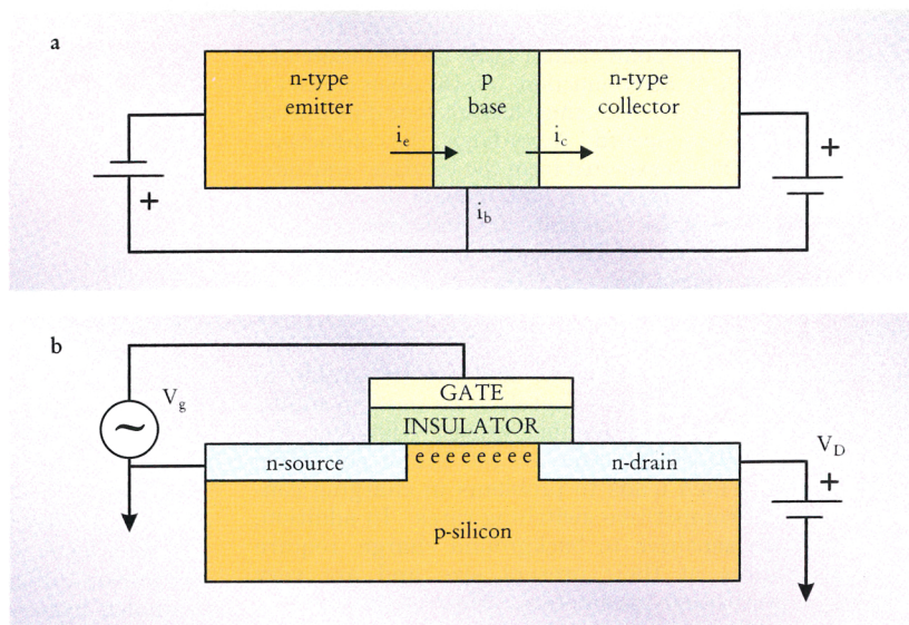
FIGURE 2. BIPOLAR AND FIELD-EFFECT TRANSISTORS. The bipolar transistor (a) functions by emitting electrons across a low-impedance, forward-biased emitter junction into the base region. Most of the electrons are collected by the high-impedance reverse-biased collector junction. The field-effect transistor (b) operates by biasing the gate to induce the presence of electrons in the "channel" in the silicon beneath it and to provide a conducting path between the n -doped source and drain regions.
