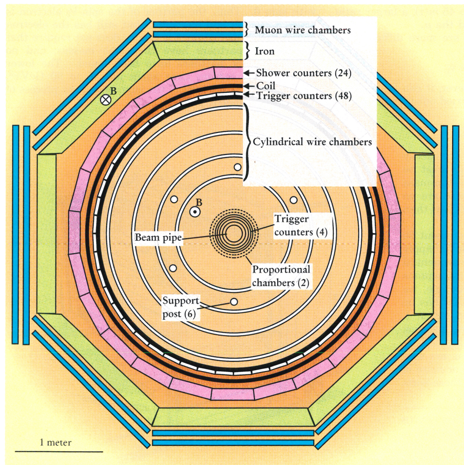
FIGURE 4. TAU DETECTION apparatus. This large-solid-angle detector, built by a team from the Stanford Linear Accelerator Center and Lawrence Berkeley National Laboratory, played a key role in the discovery of the tau.
