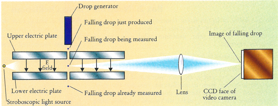
FIGURE 5. FRACTIONAL CHARGE detection scheme, showing apparatus being used to search for massive leptons or other massive particles possessing fractional electric charge. Small liquid drops, 7 \mu\text{m} in diameter, fall through air. The air resistance and the small drop size cause the drops to rapidly attain a terminal velocity proportional to the force on the drop. A vertical electric field that periodically changes direction makes it possible to measure two terminal velocities, one for each electric field direction. The difference of the two terminal velocities is proportional to the charge on the drop. The sum of the two terminal velocities is proportional to the drop mass.
