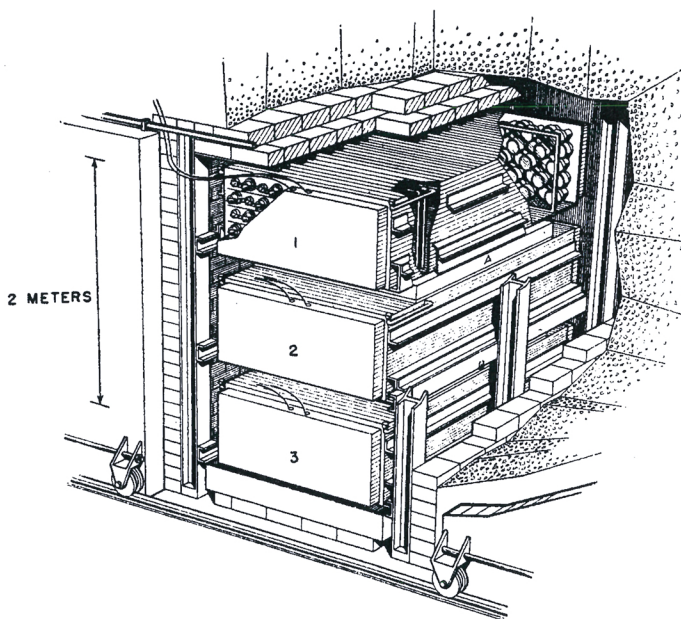
FIGURE 3. LIQUID SCINTILLATOR APPARATUS used by Frederick Reines and Clyde Cowan to detect the electron antineutrino. (From ref. 7, 1960.)
