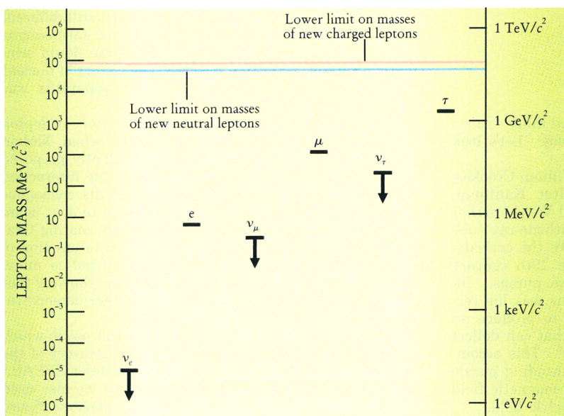
FIGURE 2. LEPTON MASSES. This logarithmic plot shows the masses of the charged leptons and upper limits on the masses of the neutrinos. There is no lower limit from experiment on the neutrino masses—indeed, they might be zero. The mass unit \text{MeV}/c^2 is equivalent to 1.8 \times 10^{-30} kg.
