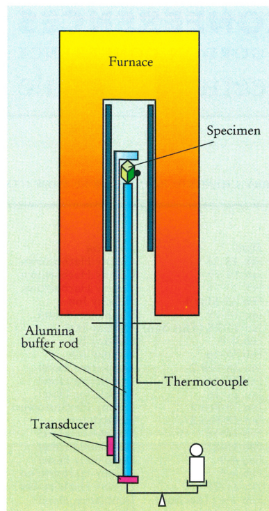
HIGH-TEMPERATURE RUS measurements can be made using a modified apparatus which holds the sample between two alumina buffer rods in a furnace. a: The piezoelectric disks are attached to the buffer rods outside the furnace and couple to the sample through the rods. Measurements can be made at temperatures up to 1825 kelvins. b: Because the resonances of the rods are dense and highly damped, they form a continuous background against which the sample resonances stand out as sharp peaks. This permits high-precision determinations of elastic constants even at high temperatures. The peaks are labeled using the mode classification scheme from ref. 7. (Adapted from ref. 13.) FIGURE 5
