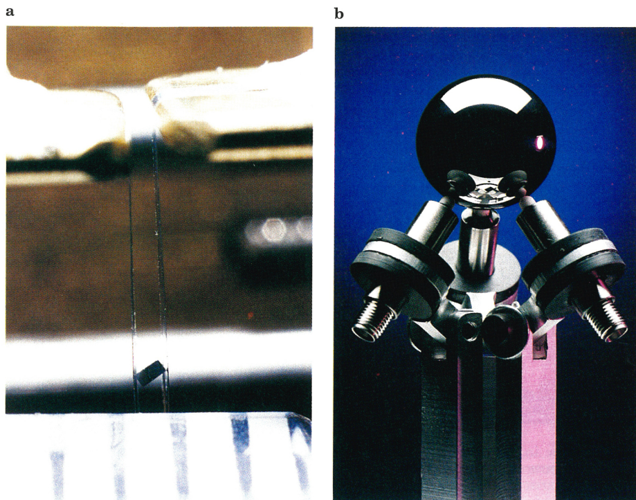
RUS MEASUREMENTS can be taken for a variety of samples and with a variety of apparatus. a: A device using thin piezoelectric films has been used to measure samples with masses down to 70 micrograms. In this photo, the space between divisions on the scale is 1 millimeter. (From ref. 17.) b: RUS has also been used to detect defects in ball bearings several centimeters in diameter. (Courtesy of Quatro Corporation, Albuquerque, New Mexico.) FIGURE 1
