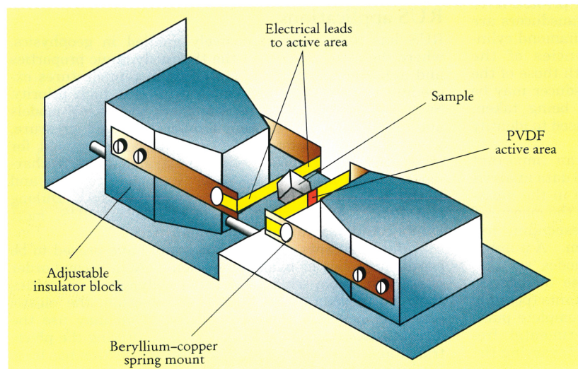
SIMPLE RUS APPARATUS holds a rectangular parallelepiped sample lightly at its corners between two 9- \mu\text{m} -thick piezoelectric-film (PVDF) transducers. One transducer excites the vibration of the sample; the other monitors the sample response and detects resonance frequencies. Samples may be as small as a few hundred microns. (Adapted from ref. 10.) FIGURE 3
