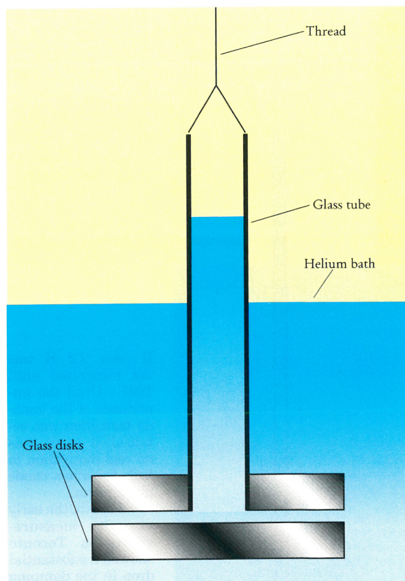
CHANNEL-FLOW SCHEME by Peter Kapitza in Moscow to measure the viscosity of helium II. Kapitza raised the optically flat glass disks and glass tube from the helium bath by means of the thread. The viscosity was measured by the pressure drop when the liquid flowed through the narrow gap between the disks. The pressure difference was given by the height of the liquid column in the glass tube. Above the lambda transition temperature T_\lambda a level difference could be observed for several minutes. Below T_\lambda the difference disappeared in seconds, leading Kapitza to conclude that the viscosity of helium II was at least 1500 times less than that of helium I. FIGURE 5
