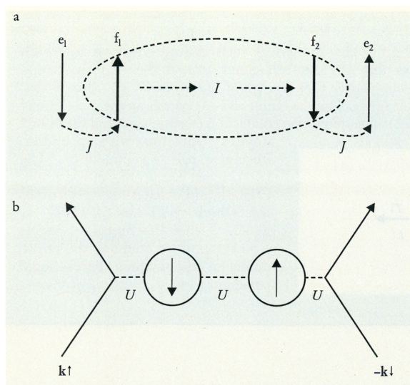
ANTIFERROMAGNETICALLY MEDIATED PAIRING in exotic superconductors. a: A real-space picture assuming that the mobile electrons pair through exchange of a spin fluctuation in the localized moment system. Exchange coupling J of electron e_1 to the local moment on site f_1 polarizes that moment. Through the antiferromagnetic exchange coupling I , this spin polarizes the second site f_2 , making it a favorable location for another electron, e_2 . Since two spin flips are involved, the process is a two-magnon one. For the cuprates the mobile carriers could be oxygen holes, and the local moments reside on copper sites. For the heavy-fermion materials the ligand atoms supply the mobile carriers, and the 4f or 5f sites supply the local moments. b: The momentum-space picture relevant to a single-band Hubbard model. Again, two spin polarizations are required to mediate a pairing interaction. FIGURE 5
