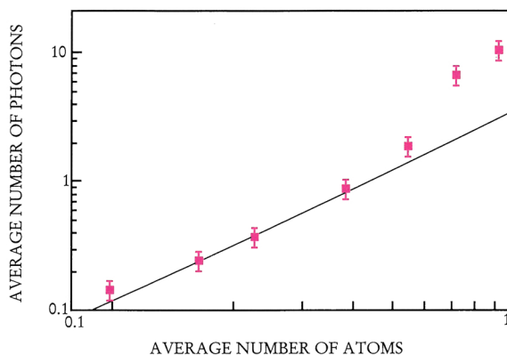
NUMBER OF PHOTONS at equilibrium versus the number of atoms in the high- Q cavity of a single-atom laser as an atomic beam passes through. Photons leaking from the mirrored ends of the cavity constitute the laser beam. Solid curve is the prediction of a one-atom quantized field model. (Adapted from ref. 1.)
