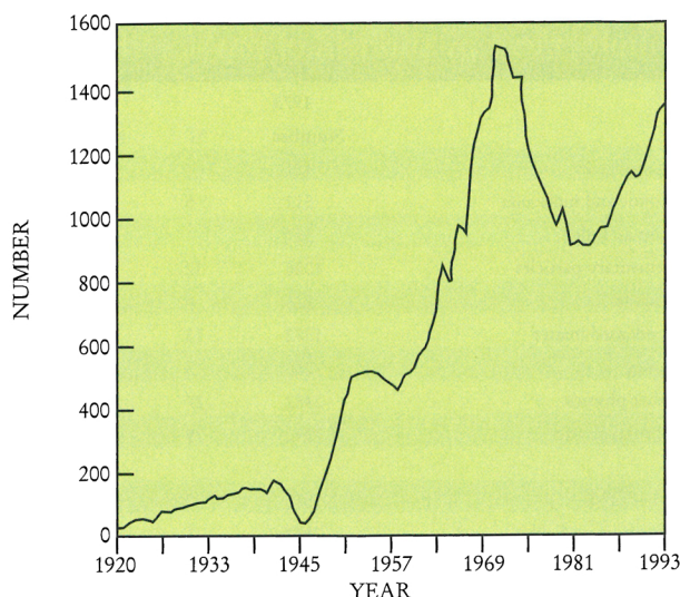
NUMBER OF PHYSICS PhDs conferred in the US from 1920 to 1993. Note the near-exponential growth until about 1970. (From reference 10.) FIGURE 2
