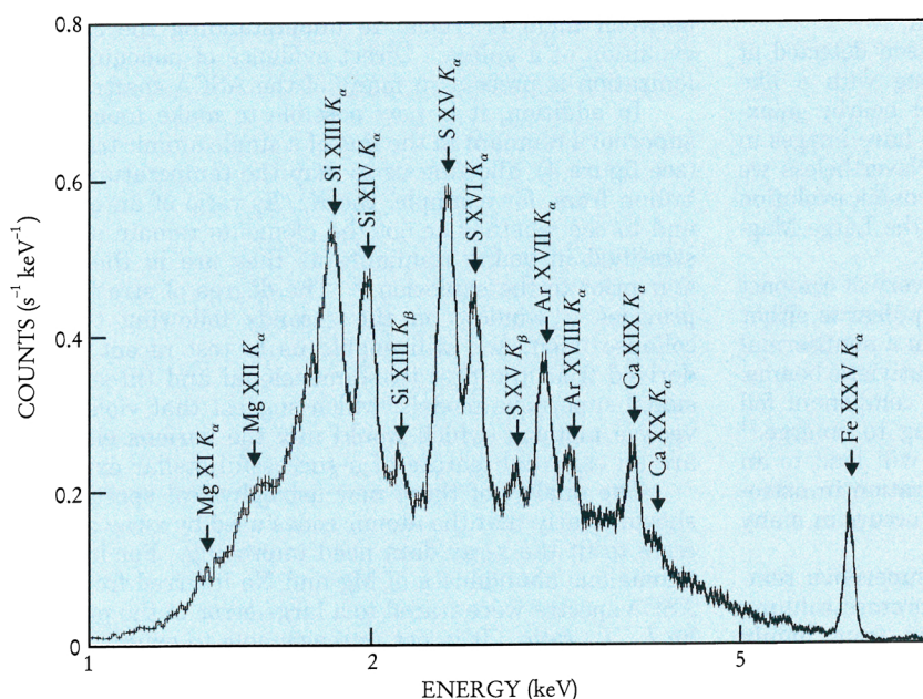
SPECTRUM of the young Milky Way supernova remnant W49, as measured by the CCD camera on the Advanced Satellite for Cosmology and Astronomy. (Adapted from reference 18.) FIGURE 3
