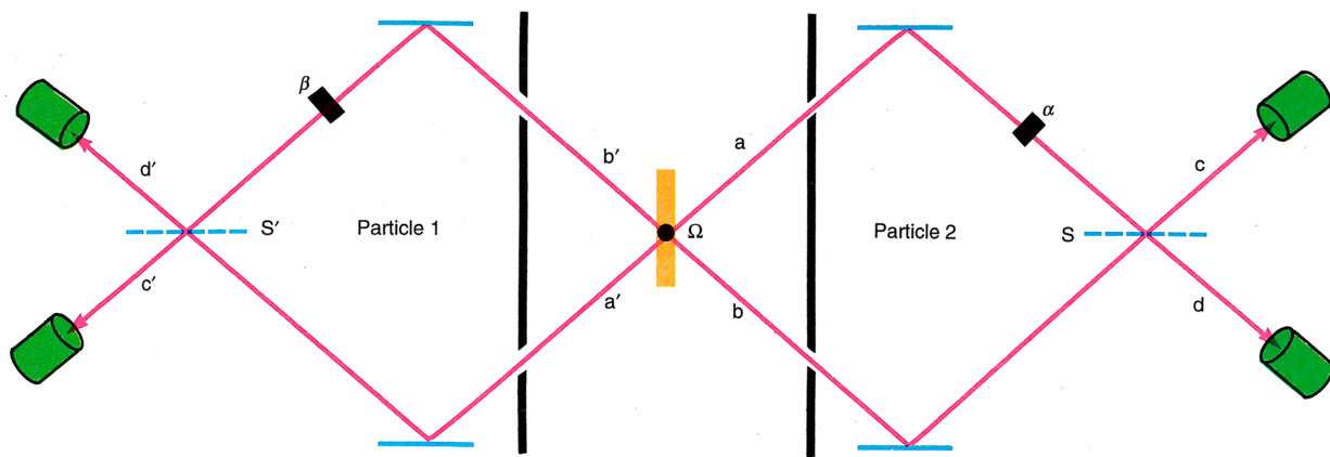
Beam splitters (half-silvered mirrors, represented by dashed blue lines) can be used in two-particle interferometry with localized photon detectors (green) in place of the extended detecting screens of figure 1. Particle \Omega in the central source decays into two photons. Phase shifters (black rectangles) are inserted into decay-photon beams a and b' , shifting their phases by \alpha and \beta , respectively. Before arriving at the detectors the alternative-path beams are mixed by the beam splitters at S and S' . Figure 2
