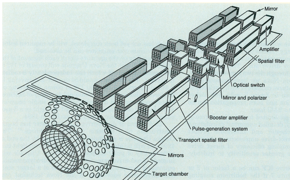
The Nova upgrade at Lawrence Livermore has been proposed as the national ignition facility, at which ignition and modest-gain ICF targets would be demonstrated. One half of the laser and target chamber is shown. Figure 8
