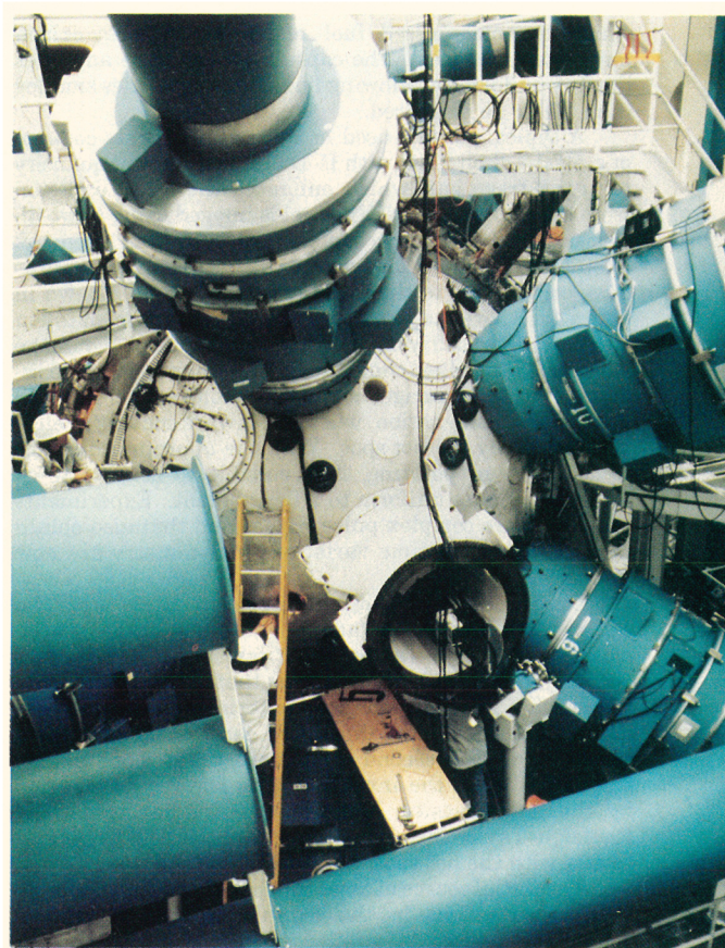
Nova target chamber. When in operation, ten laser beams deliver up to a total of 40 kJ of light in a 1-nsec pulse onto a target within this 16-foot-diameter aluminum sphere. Figure 3
