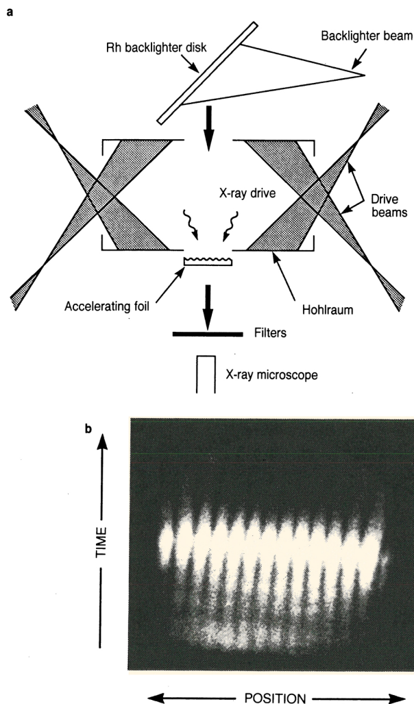
Rayleigh-Taylor instability experiment with x-ray-driven implosion. a: The experimental setup. Sinusoidal thickness variations on the foil seed the R-T instability. b: One-dimensional, continuously time-resolved data. c: Difference in logarithm of exposure between the thin and thick regions of a planar target driven by x rays. Fourier decomposition of the data (solid lines) shows modulations up to the fourth harmonic. Initial perturbation amplitude (peak to peak) and wavelength are 2.1 \mu\text{m} and 100 \mu\text{m} , respectively. Dashed lines show LASNEX simulation results. Figure 5
