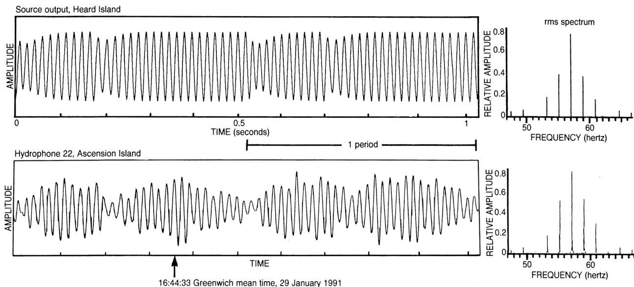
Transmitted and received signals and their spectra. Top: Transmitted signal and its spectrum as recorded at the source near Heard Island. Bottom: Signal received at Ascension Island, about 9000 km away, and its spectrum. The spectrum consists of the five strong lines of the pentaline code; half the power is in the 57-Hz carrier. (Figure courtesy of David Palmer, Atlantic Oceanographic Marine Laboratory, National Oceanic and Atmospheric Administration.) Figure 4
