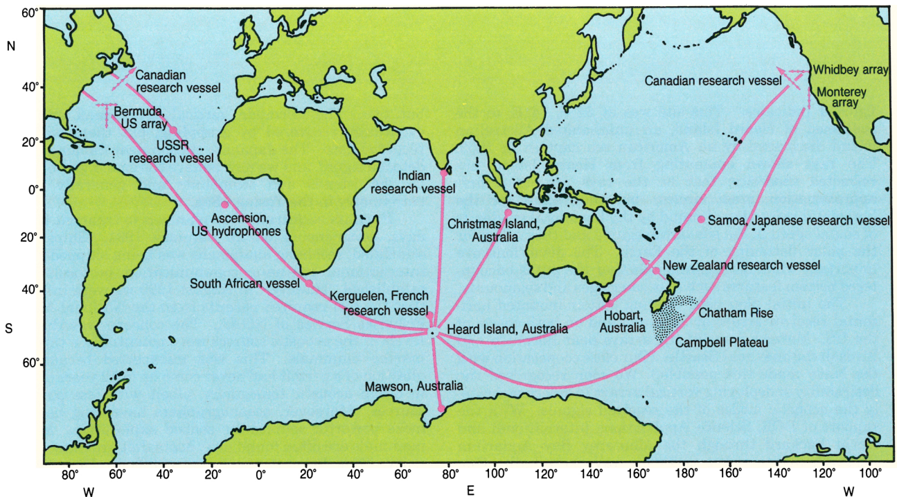
Paths taken by sound in the Heard Island feasibility test. The sources were suspended from the center well of the R/V Cory Chouest 50 km southeast of Heard Island. Black circles indicate receiver sites. Horizontal lines represent horizontal receiver arrays off the American west coast and off Bermuda. Vertical lines designate vertical arrays off Monterey and Bermuda. Lines with arrows off California and Newfoundland indicate Canadian towed arrays. Ray paths from the source to receivers are along refracted geodesics, which would be great circles but for the Earth's nonspherical shape and the ocean's horizontal sound speed gradients. Signals were received at all sites except the vertical array at Bermuda, which sank, and the Japanese station off Samoa. Figure 1
