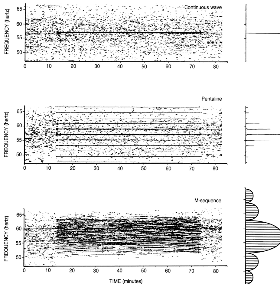
Three signal modulations and their spectra as recorded at Ascension Island. Top: 57-Hz continuous-wave tone. Middle: Pentatone code. Bottom: M-sequence pseudorandom code. These are sonograms, or time-frequency plots. Some 60-Hz noise is evident before and after the transmissions. The persistence of the lines for several minutes after the one-hour transmission stopped must be attributed to scattering and multiple horizontal paths. Figure 5
