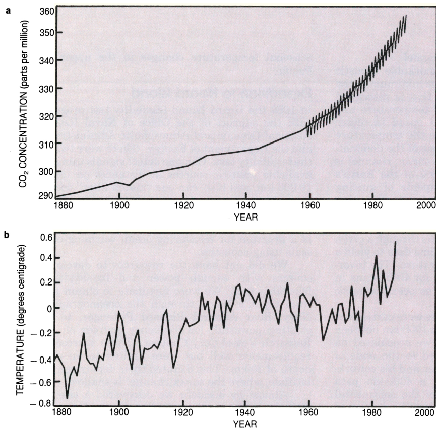
CO 2 and temperature over the last century. a: Carbon dioxide concentration in the atmosphere as determined from ice cores (smooth curve) and as measured at Mauna Loa, Hawaii (annual oscillations). 7 b: Global average surface temperature plotted as a deviation from the mean. 8 Figure 2
