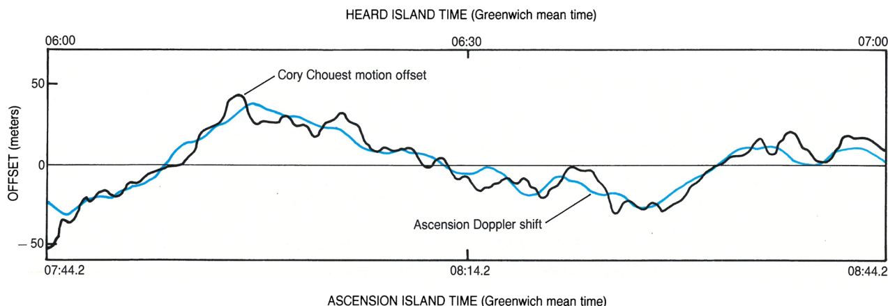
Observed and GPS phases. The black line shows the R/V Cory Chouest's departure from uniform motion along a course of 267^\circ toward Ascension Island on 26 January 1991, as determined by the Global Positioning System. The colored line is the detected phase of the signal at Ascension Island. The source-receiver separation is approximately 9000 km, yet the relative distance between them is tracked to within 10 m. Figure 7
