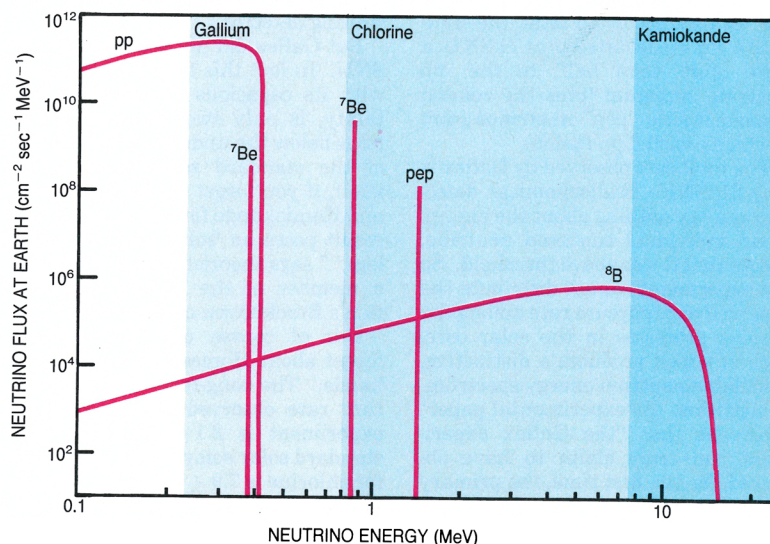
Solar neutrino spectra that contribute significantly to the signals predicted for the extant detectors, as calculated from the standard solar model. For the monoenergetic {}^7\text{Be} and pep lines, the flux is given in \text{cm}^{-2} \text{sec}^{-1} . Shadings indicate detector thresholds: Kamiokande sees only the {}^8\text{B} decay spectrum. Chlorine detectors can also see {}^7\text{Be} neutrinos. The gallium detectors, with a 233-keV threshold, are the only ones that can see the pp spectrum.
