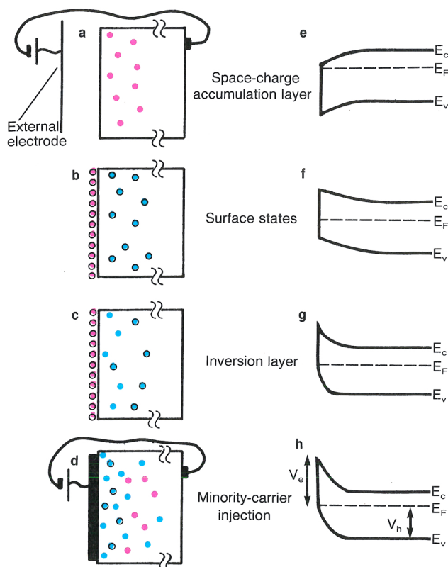
Central ideas in semiconductor surface physics, arranged in the order in which their possible roles came to be appreciated through research at Bell Telephone Laboratories between 1945 and 1947. a-d: Spatial distribution of the change in electric charge density in or on an n-type semiconductor relative to that of a uniform neutral state. Mobile electrons are indicated by red dots and mobile holes by blue dots, while charges trapped on surfaces or at centers in the bulk are indicated by dots circled in black. In a and d metal electrodes, whose charges are not shown, are connected through a battery to a contact at the rear of the semiconductor. e-h: Energies of the conduction and valence band edges versus depth; the Fermi level is indicated by a dashed line. The barriers for electron and hole motion are V_e and V_h , respectively. Infinitesimal bias is assumed in g . Figure 6
