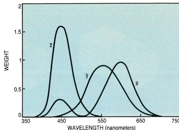
Color-matching functions \bar{x}(\lambda) , \bar{y}(\lambda) and \bar{z}(\lambda) of the CIE 1931 Standard Observer. Figure 5
